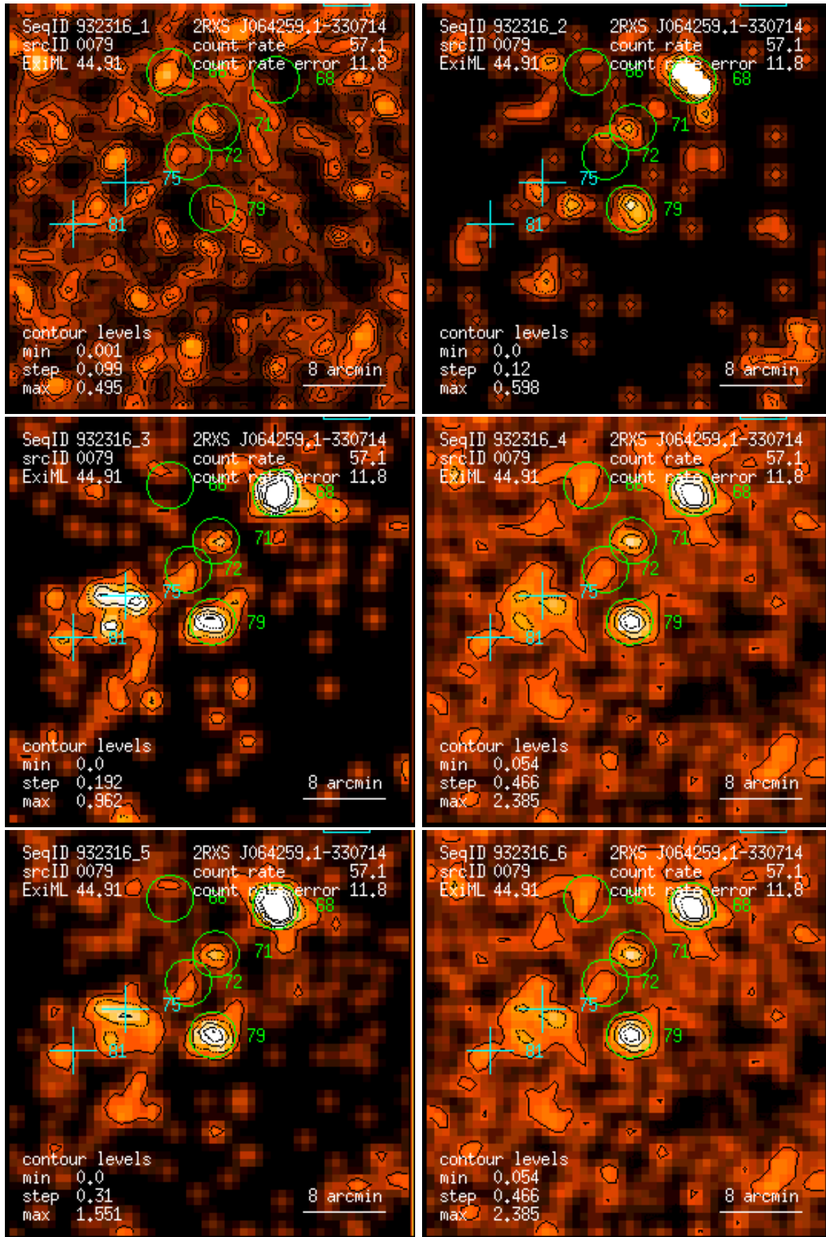
Figure 79: RASS 932316: detection 0079: band rate images, Gaussian filter: (1) PSPC channels 11 – 41, (2) 52 – 90, (3) 91 – 201, (4) 11 – 235, (5) 52 – 201, (6) 11 – 201. Broad band rates in counts/ks. Band rate contour levels in counts/ks/arcmin 2 .
