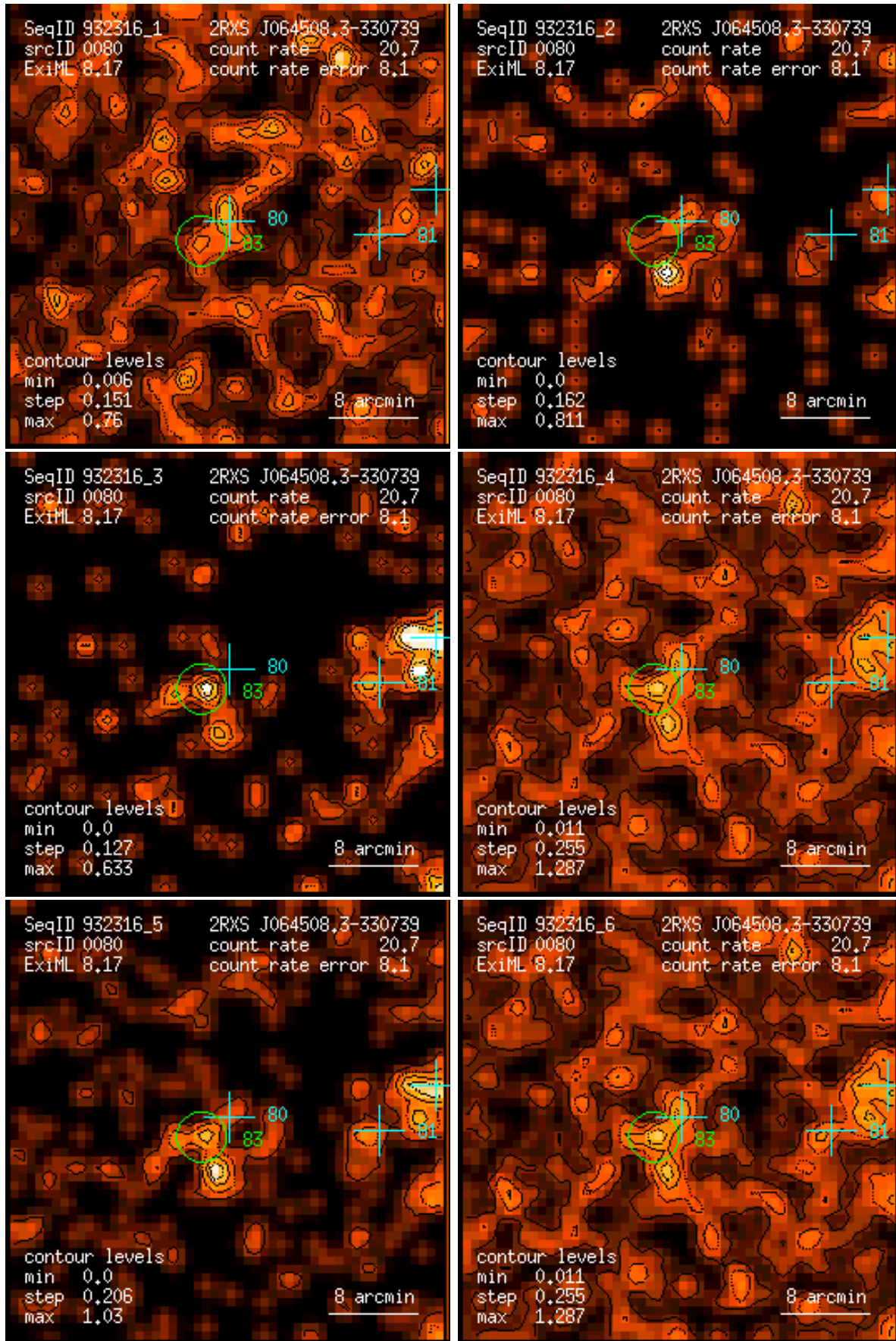
Figure 80: RASS 932316: detection 0080: band rate images, Gaussian filter: (1) PSPC channels 11 – 41, (2) 52 – 90, (3) 91 – 201, (4) 11 – 235, (5) 52 – 201, (6) 11 – 201. Broad band rates in counts/ks. Band rate contour levels in counts/ks/arcmin 2 .
