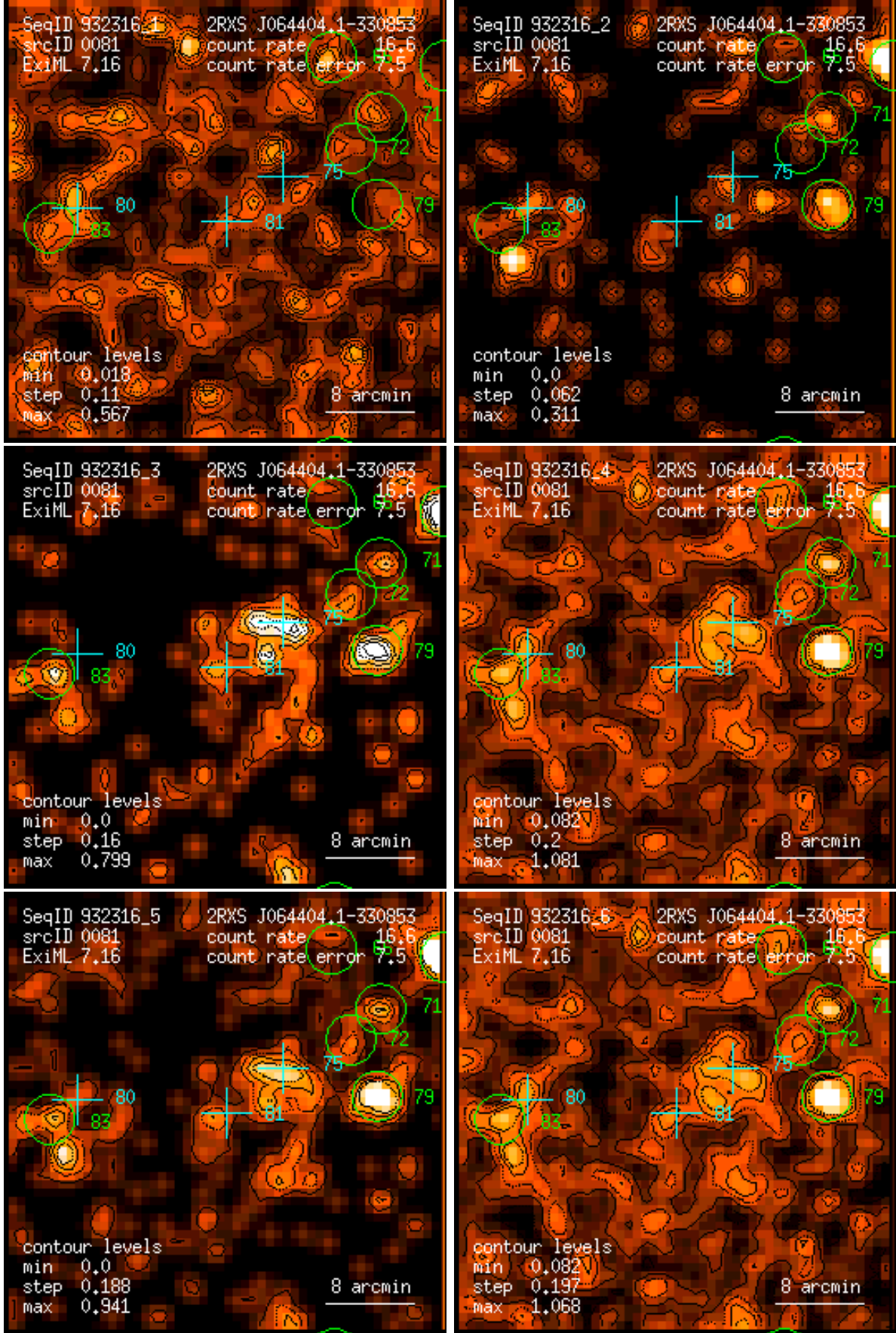
Figure 81: RASS 932316: detection 0081: band rate images, Gaussian filter: (1) PSPC channels 11 – 41, (2) 52 – 90, (3) 91 – 201, (4) 11 – 235, (5) 52 – 201, (6) 11 – 201. Broad band rates in counts/ks. Band rate contour levels in counts/ks/arcmin 2 .
