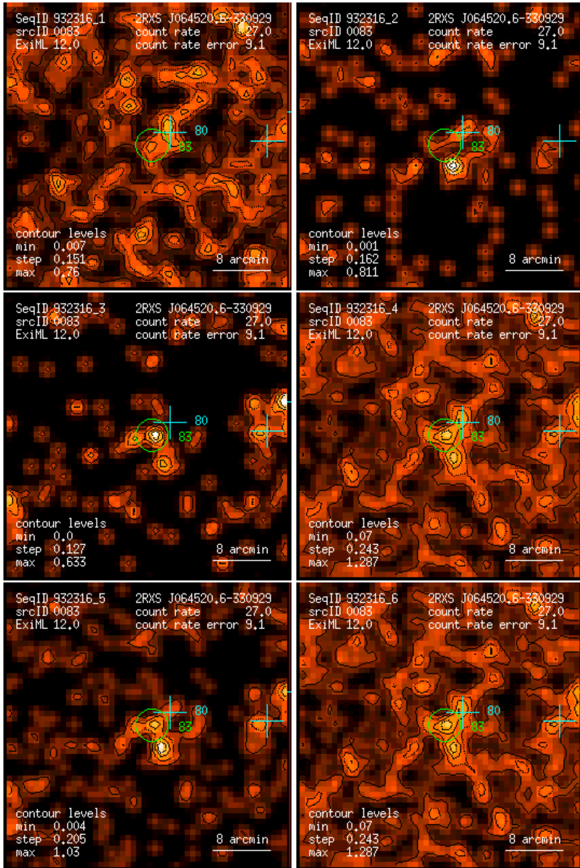
Figure 83: RASS 932316: detection 0083: band rate images, Gaussian filter: (1) PSPC channels 11 – 41, (2) 52 – 90, (3) 91 – 201, (4) 11 – 235, (5) 52 – 201, (6) 11 – 201. Broad band rates in counts/ks. Band rate contour levels in counts/ks/arcmin 2 .
