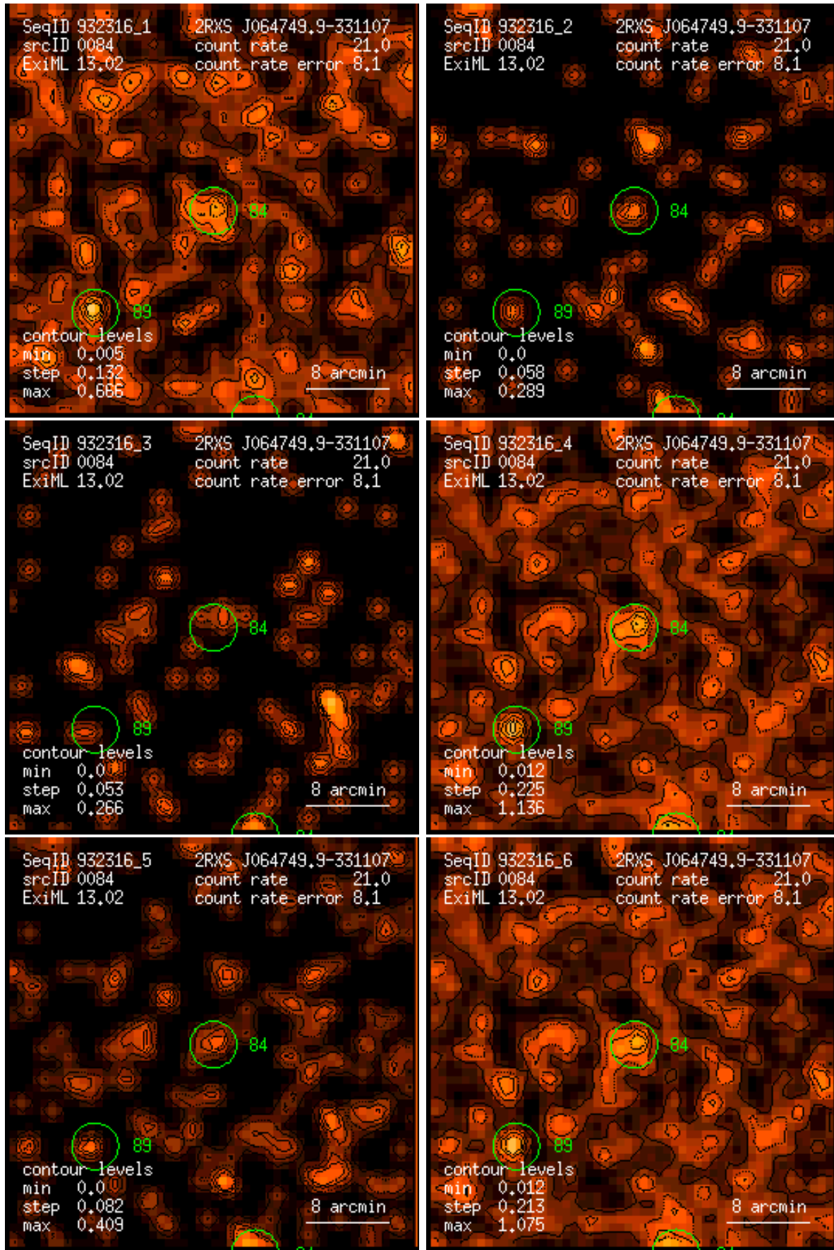
Figure 84: RASS 932316: detection 0084: band rate images, Gaussian filter: (1) PSPC channels 11 – 41, (2) 52 – 90, (3) 91 – 201, (4) 11 – 235, (5) 52 – 201, (6) 11 – 201. Broad band rates in counts/ks. Band rate contour levels in counts/ks/arcmin 2 .
