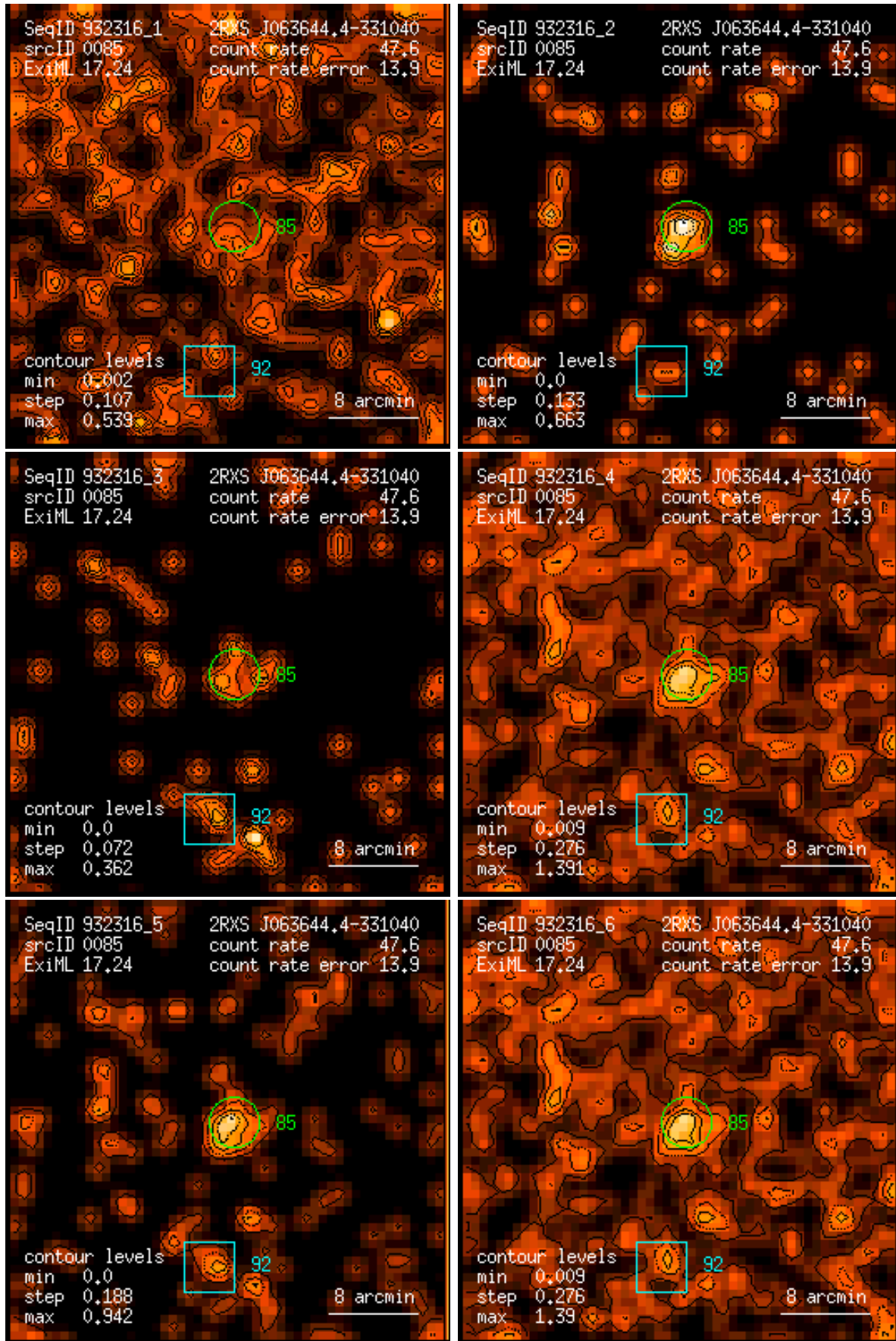
Figure 85: RASS 932316: detection 0085: band rate images, Gaussian filter: (1) PSPC channels 11 – 41, (2) 52 – 90, (3) 91 – 201, (4) 11 – 235, (5) 52 – 201, (6) 11 – 201. Broad band rates in counts/ks. Band rate contour levels in counts/ks/arcmin 2 .
