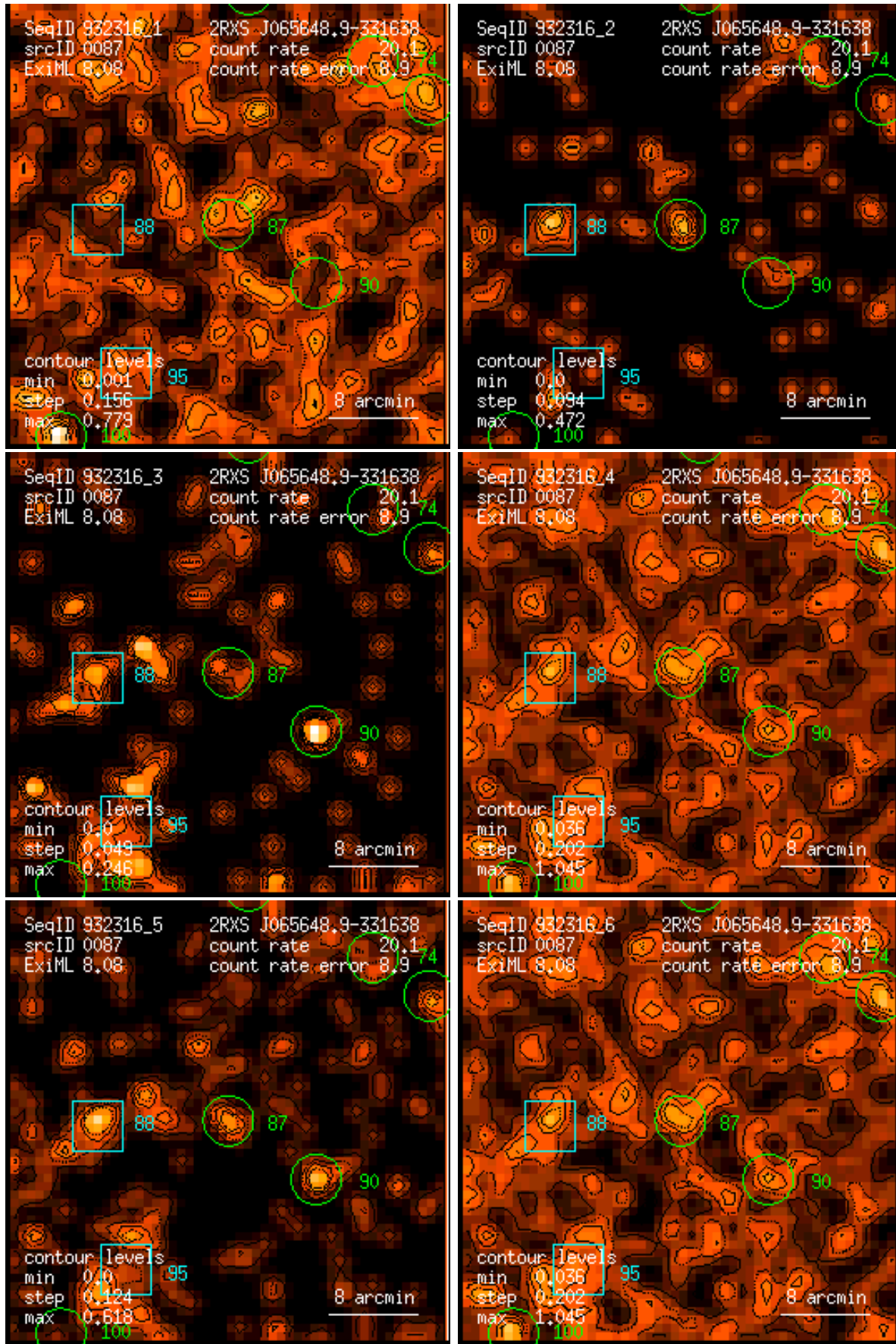
Figure 87: RASS 932316: detection 0087: band rate images, Gaussian filter: (1) PSPC channels 11 – 41, (2) 52 – 90, (3) 91 – 201, (4) 11 – 235, (5) 52 – 201, (6) 11 – 201. Broad band rates in counts/ks. Band rate contour levels in counts/ks/arcmin 2 .
