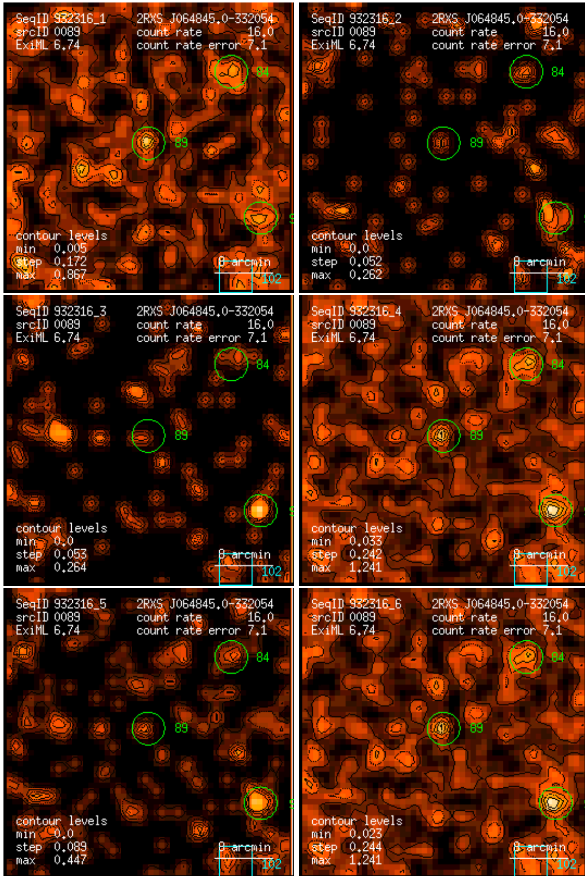
Figure 89: RASS 932316: detection 0089: band rate images, Gaussian filter: (1) PSPC channels 11 – 41, (2) 52 – 90, (3) 91 – 201, (4) 11 – 235, (5) 52 – 201, (6) 11 – 201. Broad band rates in counts/ks. Band rate contour levels in counts/ks/arcmin 2 .
