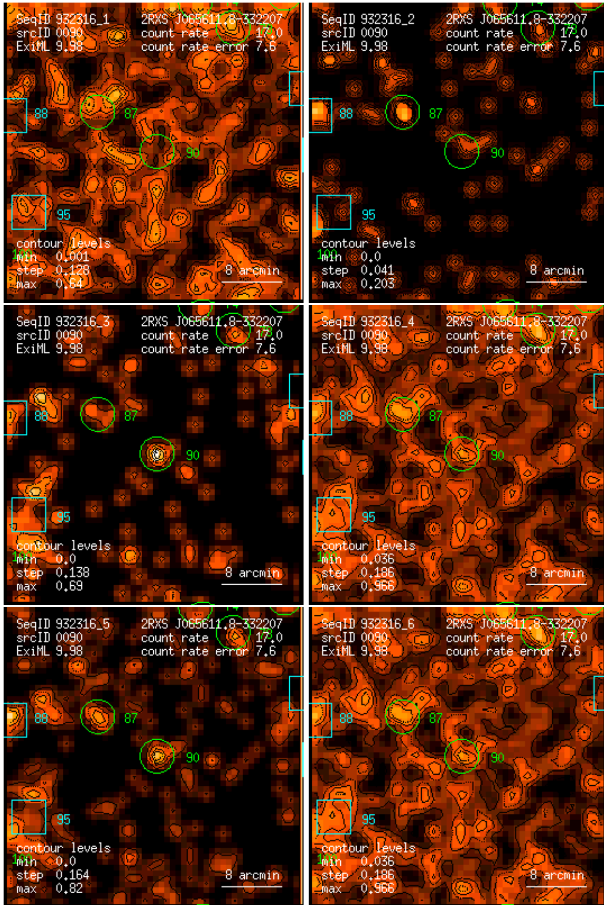
Figure 90: RASS 932316: detection 0090: band rate images, Gaussian filter: (1) PSPC channels 11 – 41, (2) 52 – 90, (3) 91 – 201, (4) 11 – 235, (5) 52 – 201, (6) 11 – 201. Broad band rates in counts/ks. Band rate contour levels in counts/ks/arcmin 2 .
