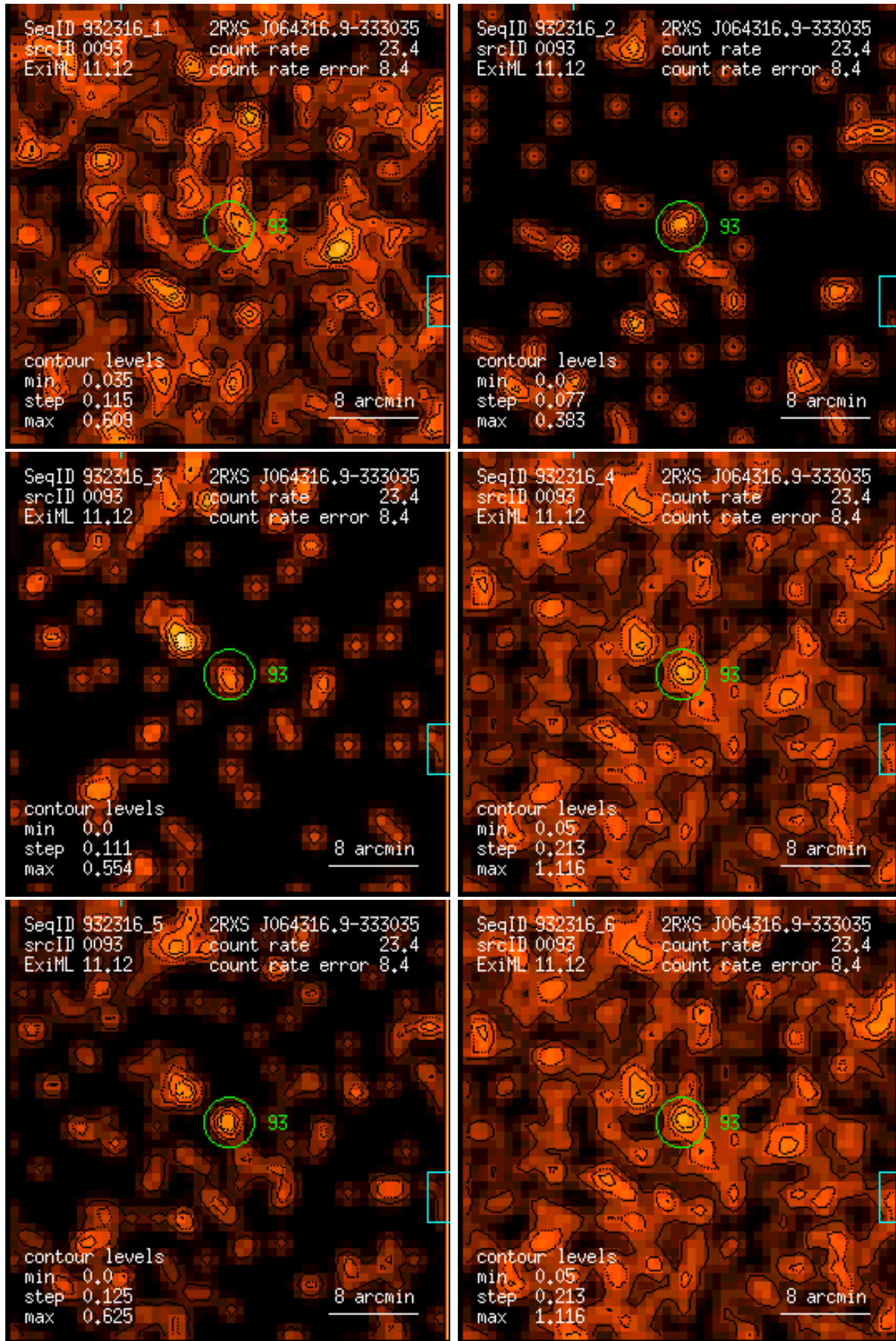
Figure 93: RASS 932316: detection 0093: band rate images, Gaussian filter: (1) PSPC channels 11 – 41, (2) 52 – 90, (3) 91 – 201, (4) 11 – 235, (5) 52 – 201, (6) 11 – 201. Broad band rates in counts/ks. Band rate contour levels in counts/ks/arcmin 2 .
