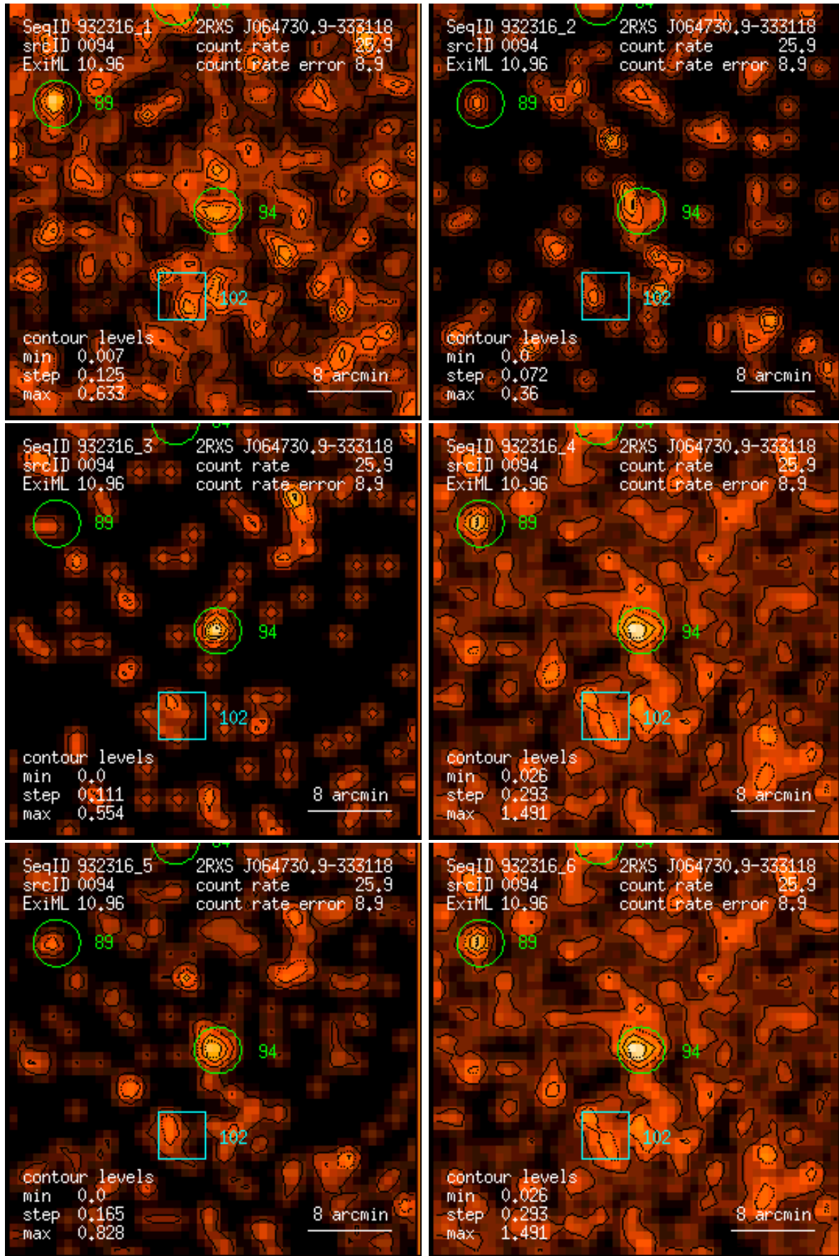
Figure 94: RASS 932316: detection 0094: band rate images, Gaussian filter: (1) PSPC channels 11 – 41, (2) 52 – 90, (3) 91 – 201, (4) 11 – 235, (5) 52 – 201, (6) 11 – 201. Broad band rates in counts/ks. Band rate contour levels in counts/ks/arcmin 2 .
