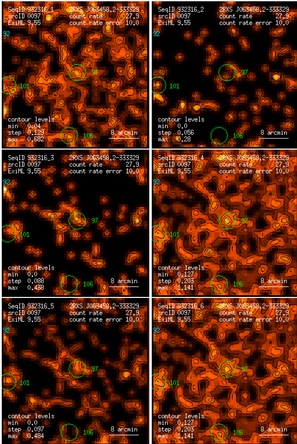
Figure 97: RASS 932316: detection 0097: band rate images, Gaussian filter: (1) PSPC channels 11 – 41, (2) 52 – 90, (3) 91 – 201, (4) 11 – 235, (5) 52 – 201, (6) 11 – 201. Broad band rates in counts/ks. Band rate contour levels in counts/ks/arcmin 2 .
