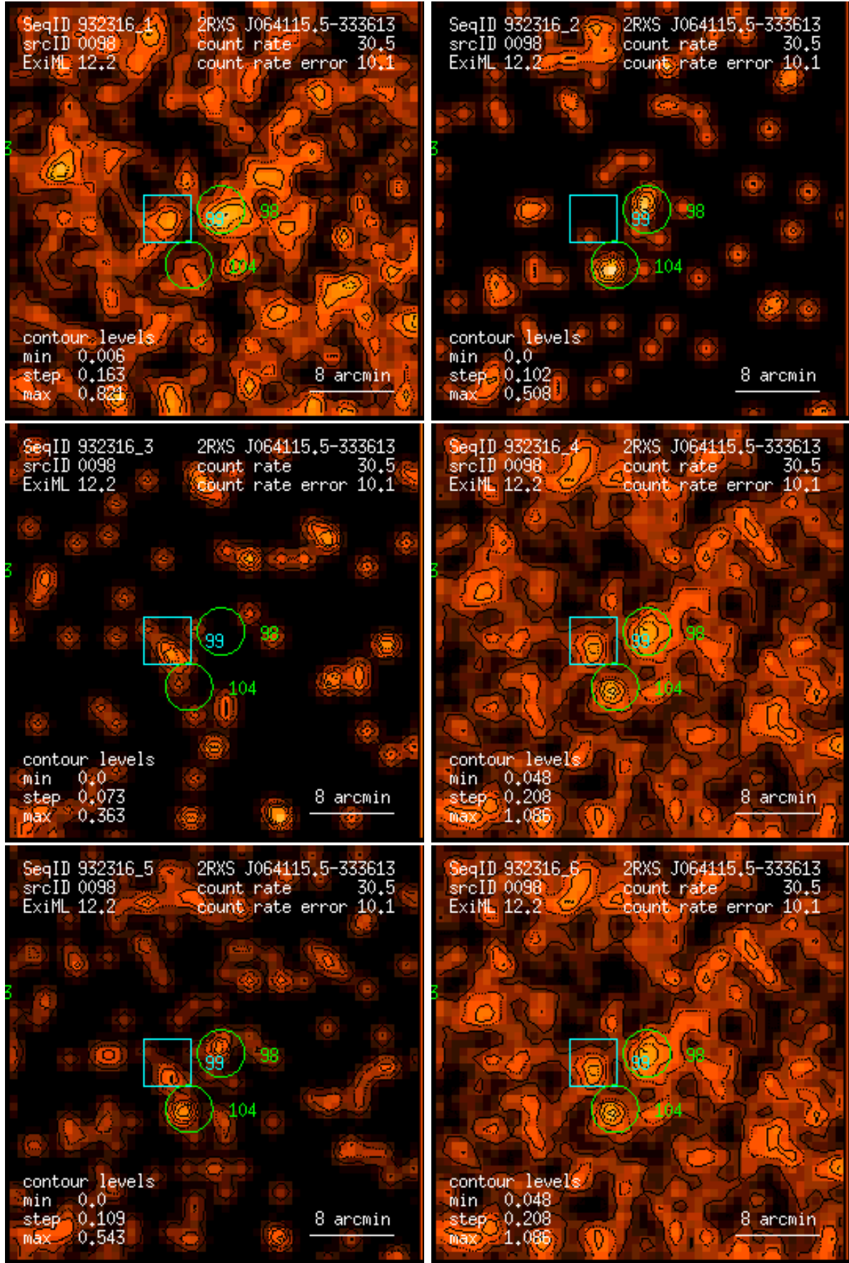
Figure 98: RASS 932316: detection 0098: band rate images, Gaussian filter: (1) PSPC channels 11 – 41, (2) 52 – 90, (3) 91 – 201, (4) 11 – 235, (5) 52 – 201, (6) 11 – 201. Broad band rates in counts/ks. Band rate contour levels in counts/ks/arcmin 2 .
