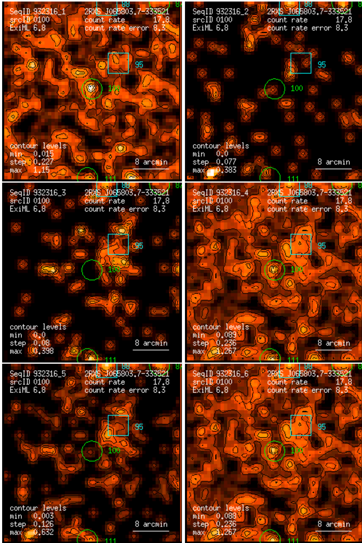
Figure 100: RASS 932316: detection 0100: band rate images, Gaussian filter: (1) PSPC channels 11 – 41, (2) 52 – 90, (3) 91 – 201, (4) 11 – 235, (5) 52 – 201, (6) 11 – 201. Broad band rates in counts/ks. Band rate contour levels in counts/ks/arcmin 2 .
