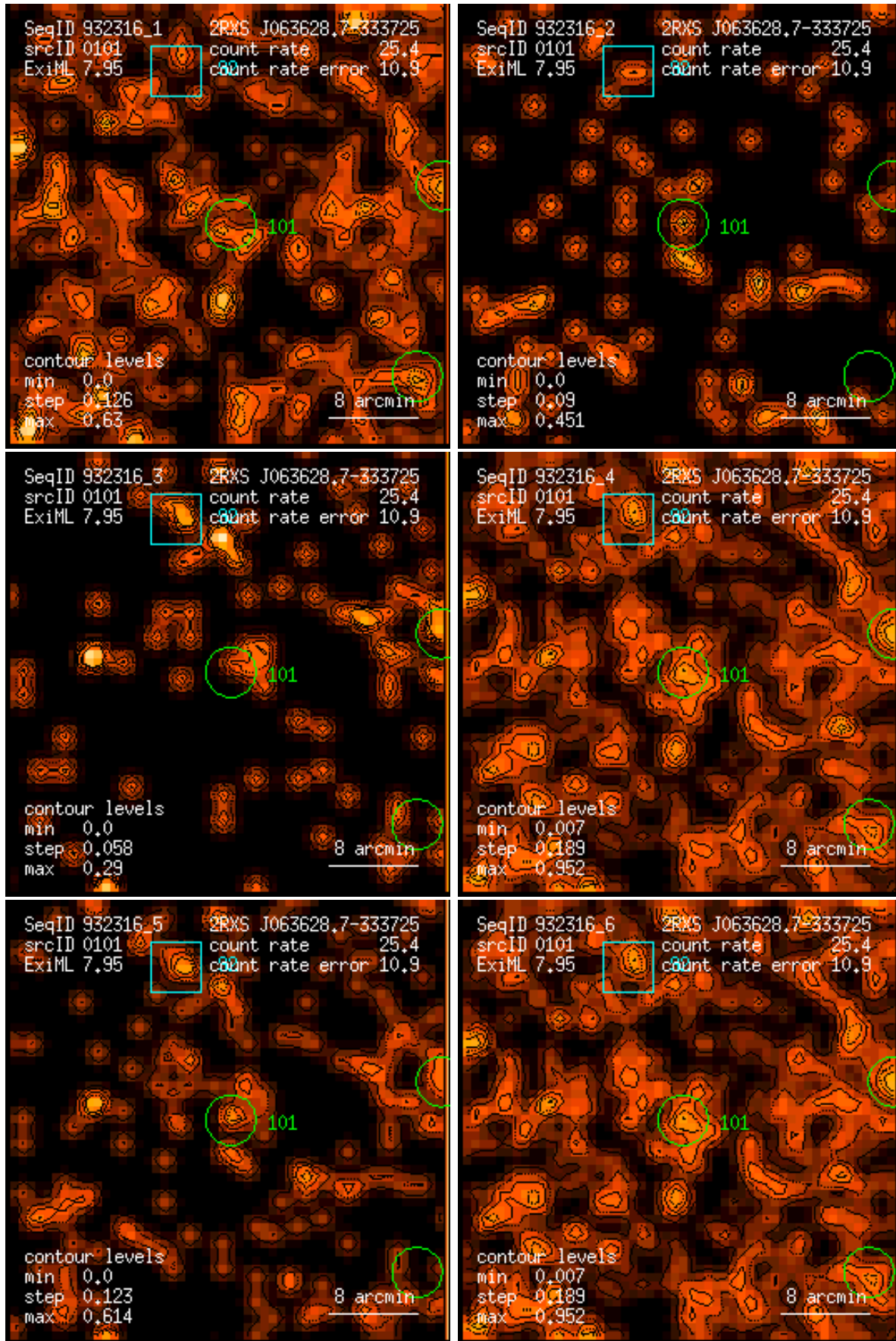
Figure 101: RASS 932316: detection 0101: band rate images, Gaussian filter: (1) PSPC channels 11 – 41, (2) 52 – 90, (3) 91 – 201, (4) 11 – 235, (5) 52 – 201, (6) 11 – 201. Broad band rates in counts/ks. Band rate contour levels in counts/ks/arcmin 2 .
