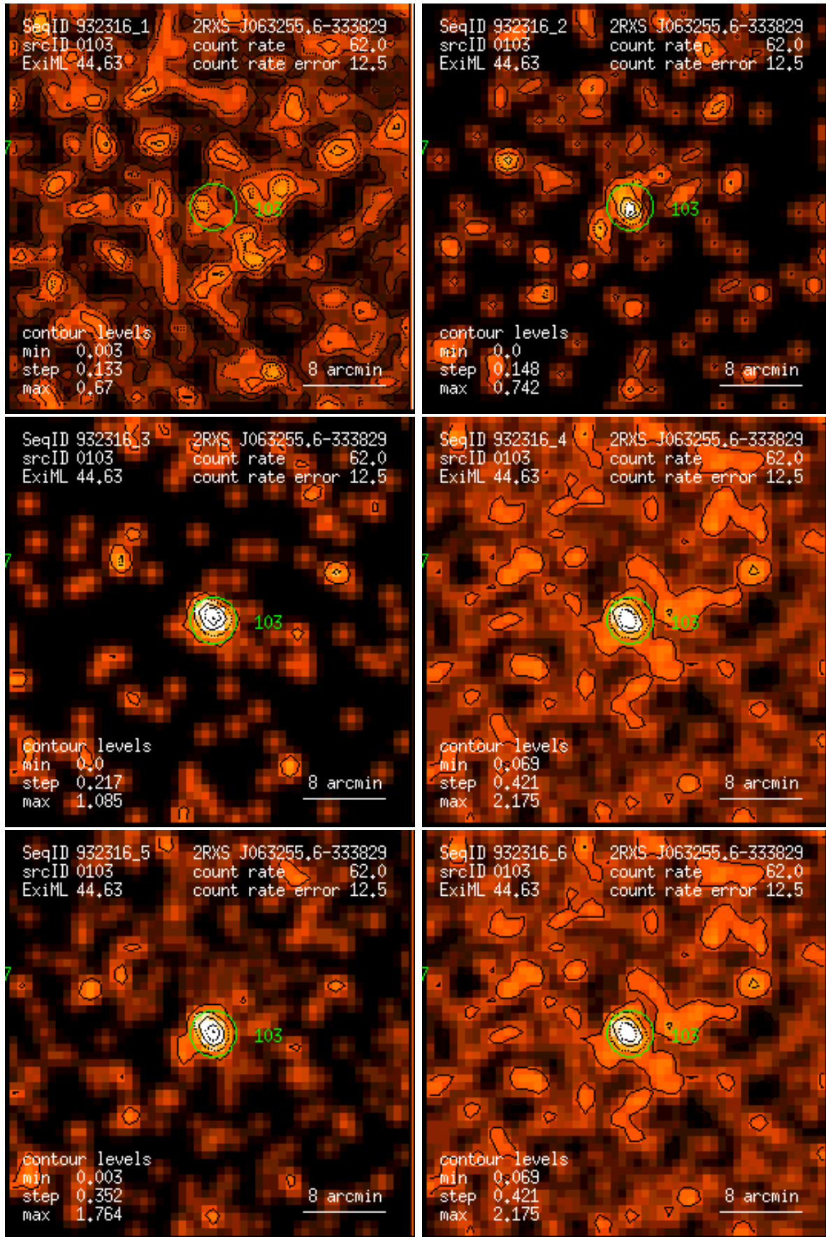
Figure 103: RASS 932316: detection 0103: band rate images, Gaussian filter: (1) PSPC channels 11 – 41, (2) 52 – 90, (3) 91 – 201, (4) 11 – 235, (5) 52 – 201, (6) 11 – 201. Broad band rates in counts/ks. Band rate contour levels in counts/ks/arcmin 2 .
