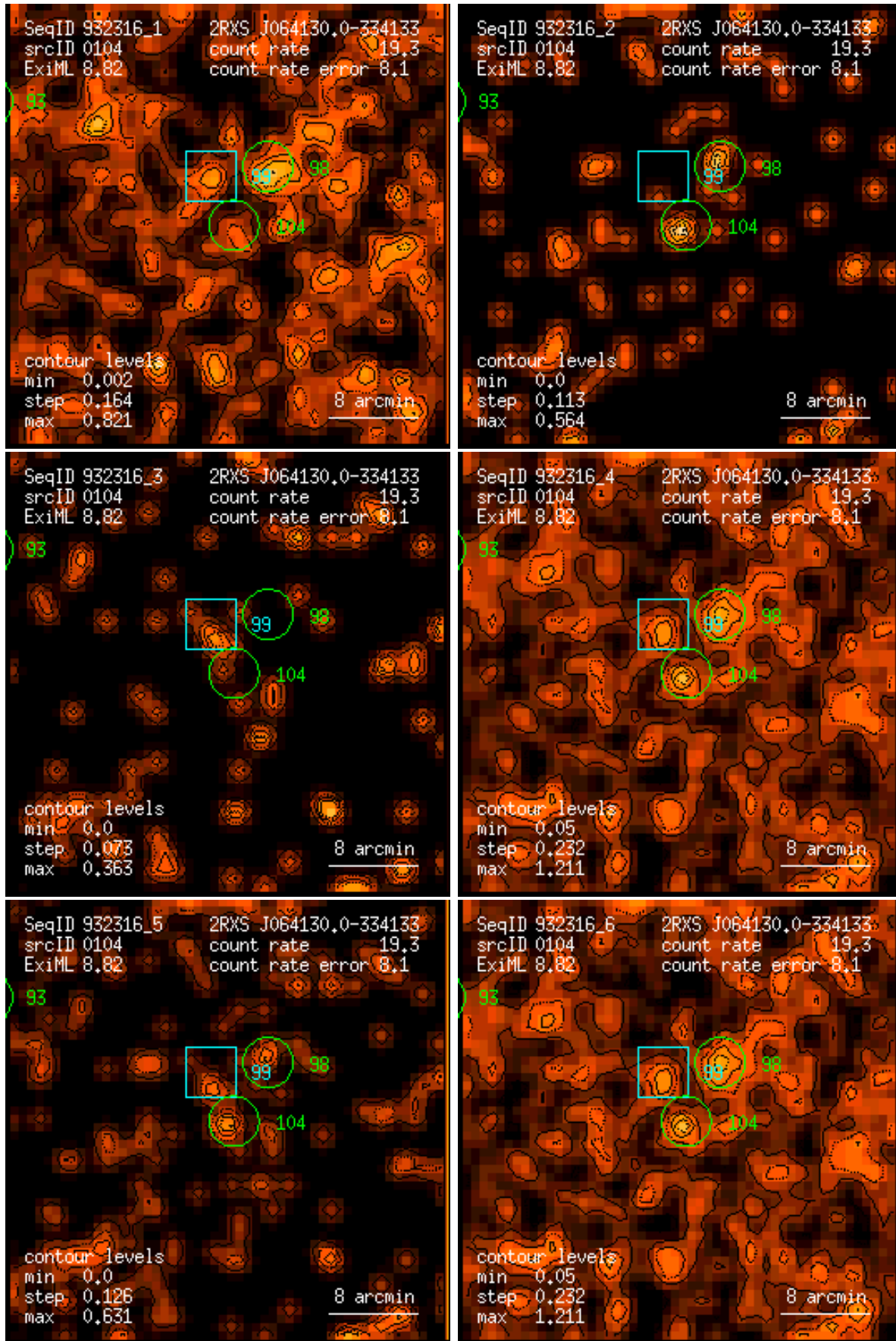
Figure 104: RASS 932316: detection 0104: band rate images, Gaussian filter: (1) PSPC channels 11 – 41, (2) 52 – 90, (3) 91 – 201, (4) 11 – 235, (5) 52 – 201, (6) 11 – 201. Broad band rates in counts/ks. Band rate contour levels in counts/ks/arcmin 2 .
