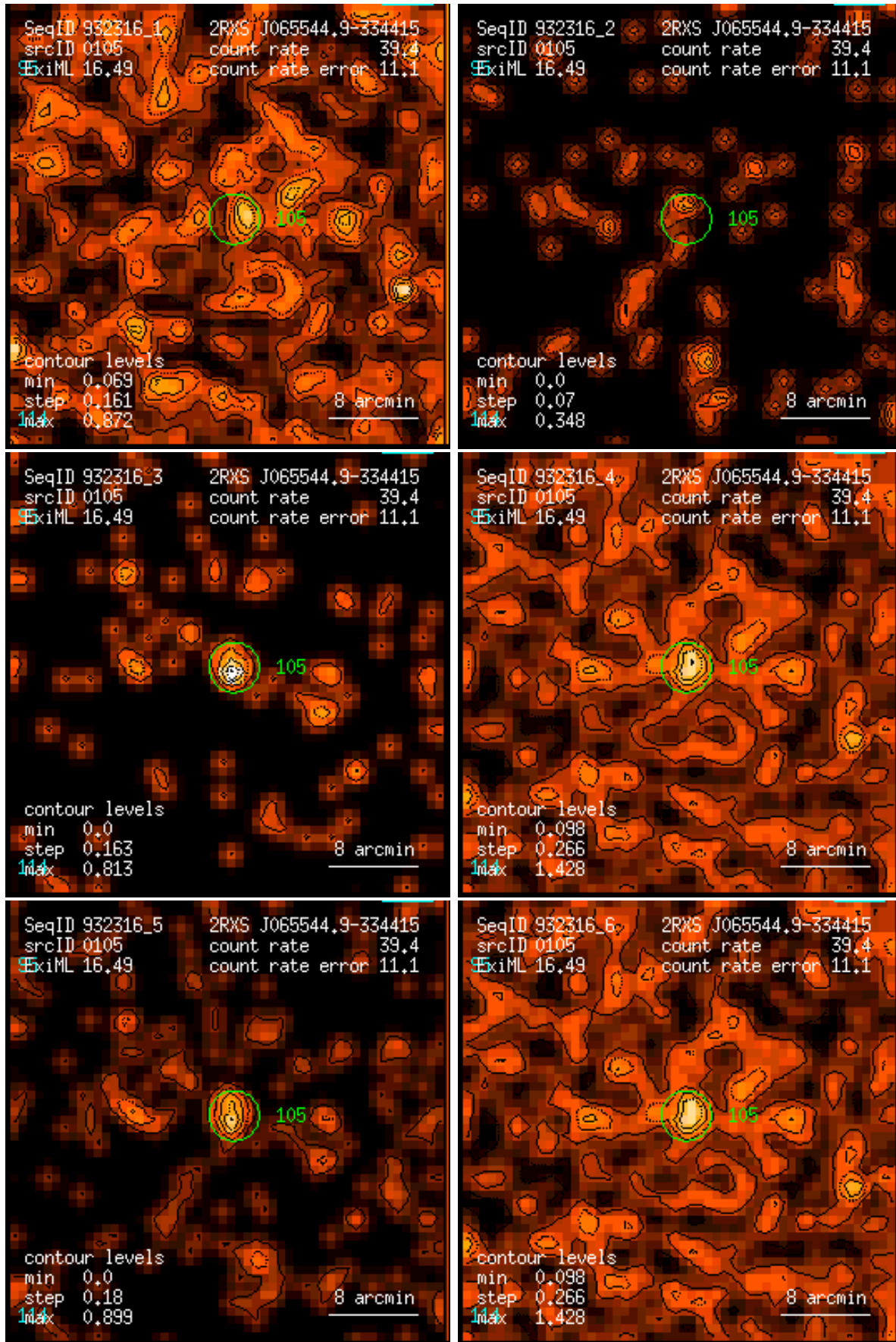
Figure 105: RASS 932316: detection 0105: band rate images, Gaussian filter: (1) PSPC channels 11 – 41, (2) 52 – 90, (3) 91 – 201, (4) 11 – 235, (5) 52 – 201, (6) 11 – 201. Broad band rates in counts/ks. Band rate contour levels in counts/ks/arcmin 2 .
