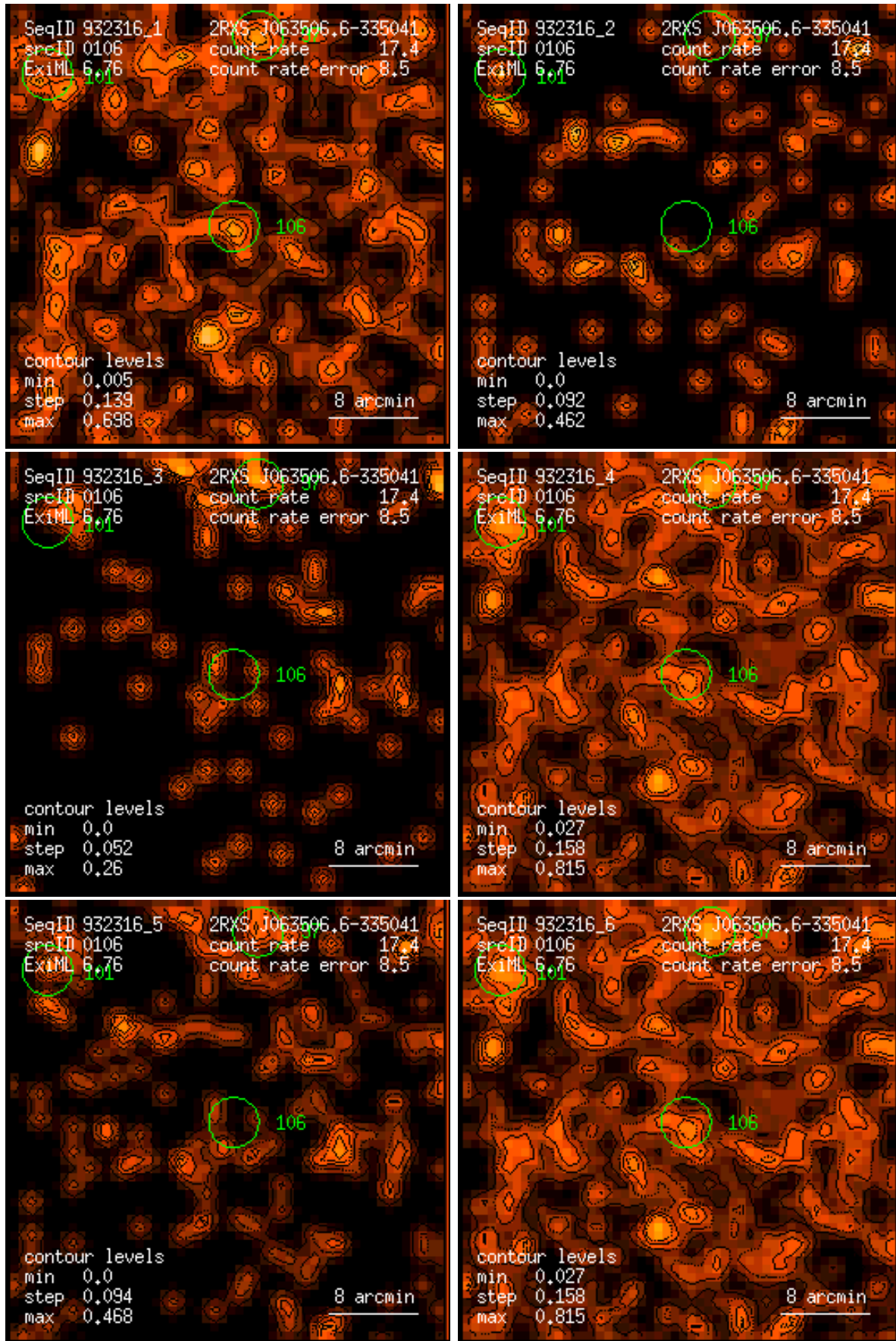
Figure 106: RASS 932316: detection 0106: band rate images, Gaussian filter: (1) PSPC channels 11 – 41, (2) 52 – 90, (3) 91 – 201, (4) 11 – 235, (5) 52 – 201, (6) 11 – 201. Broad band rates in counts/ks. Band rate contour levels in counts/ks/arcmin 2 .
