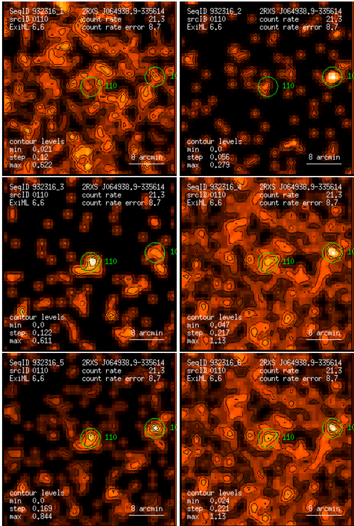
Figure 110: RASS 932316: detection 0110: band rate images, Gaussian filter: (1) PSPC channels 11 – 41, (2) 52 – 90, (3) 91 – 201, (4) 11 – 235, (5) 52 – 201, (6) 11 – 201. Broad band rates in counts/ks. Band rate contour levels in counts/ks/arcmin 2 .
