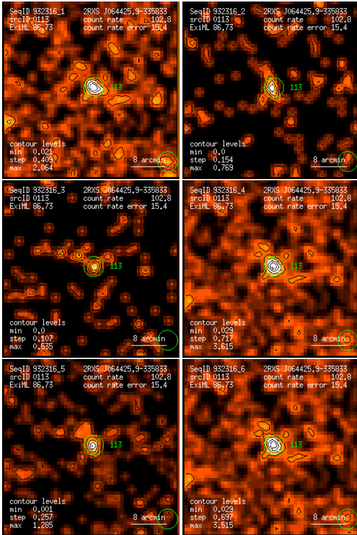
Figure 113: RASS 932316: detection 0113: band rate images, Gaussian filter: (1) PSPC channels 11 – 41, (2) 52 – 90, (3) 91 – 201, (4) 11 – 235, (5) 52 – 201, (6) 11 – 201. Broad band rates in counts/ks. Band rate contour levels in counts/ks/arcmin 2 .
