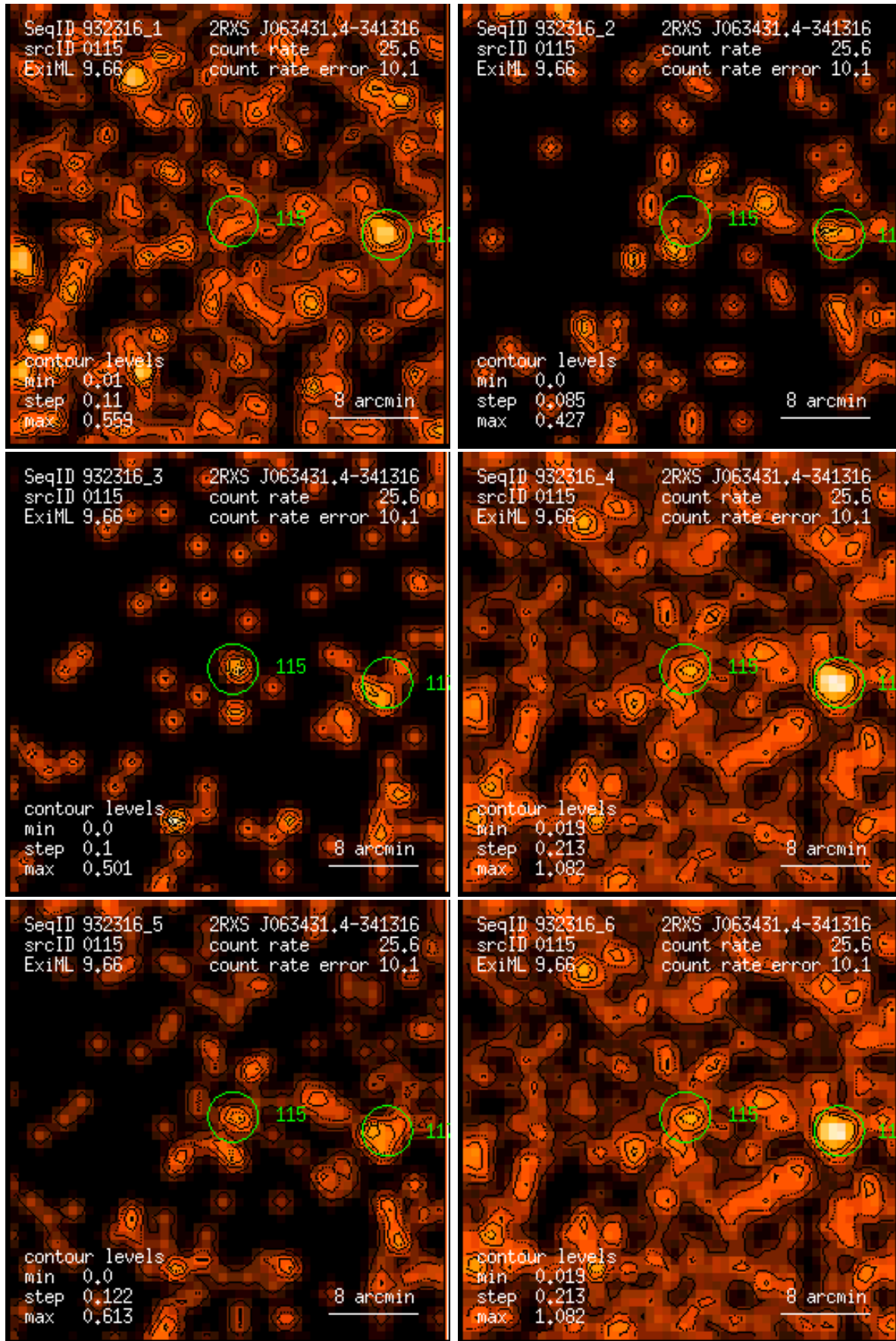
Figure 115: RASS 932316: detection 0115: band rate images, Gaussian filter: (1) PSPC channels 11 – 41, (2) 52 – 90, (3) 91 – 201, (4) 11 – 235, (5) 52 – 201, (6) 11 – 201. Broad band rates in counts/ks. Band rate contour levels in counts/ks/arcmin 2 .
