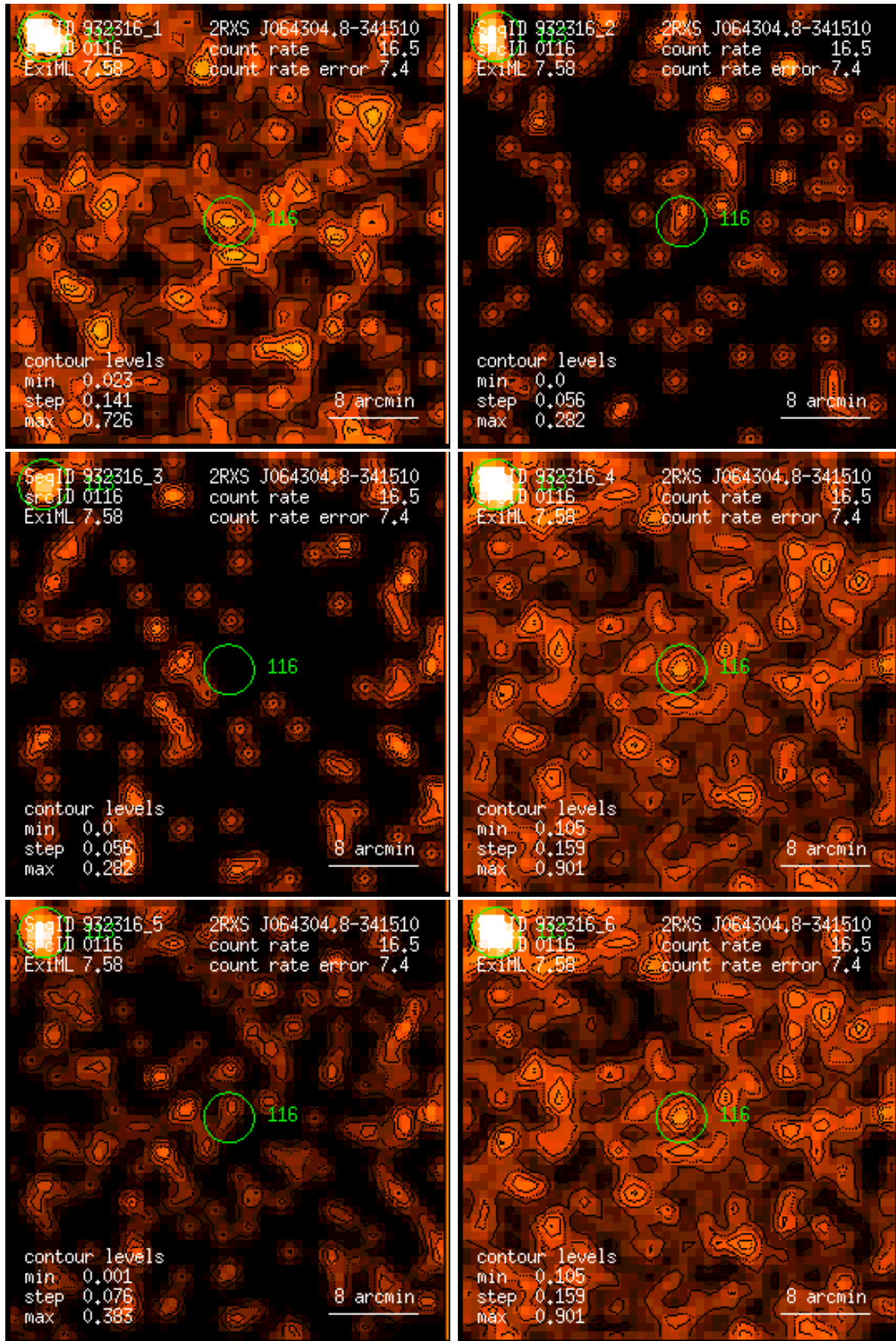
Figure 116: RASS 932316: detection 0116: band rate images, Gaussian filter: (1) PSPC channels 11 – 41, (2) 52 – 90, (3) 91 – 201, (4) 11 – 235, (5) 52 – 201, (6) 11 – 201. Broad band rates in counts/ks. Band rate contour levels in counts/ks/arcmin 2 .
