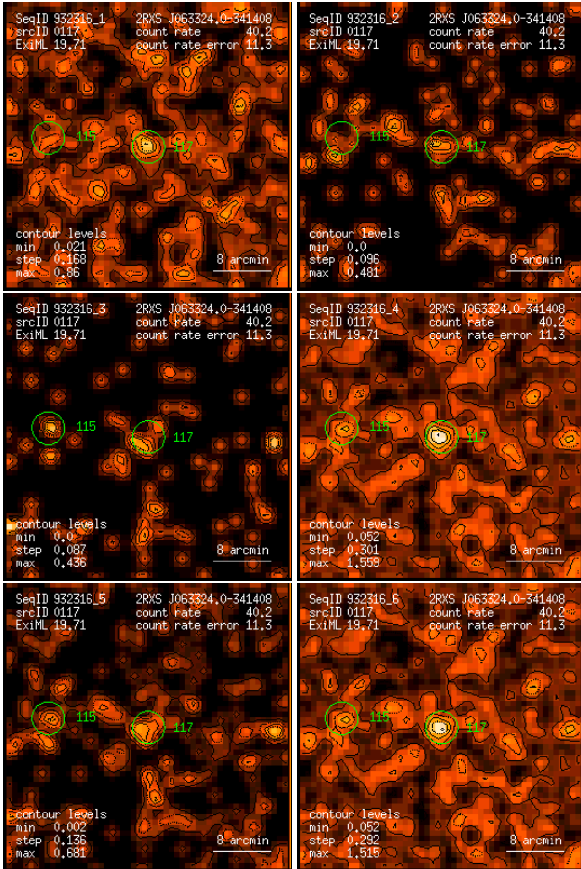
Figure 117: RASS 932316: detection 0117: band rate images, Gaussian filter: (1) PSPC channels 11 – 41, (2) 52 – 90, (3) 91 – 201, (4) 11 – 235, (5) 52 – 201, (6) 11 – 201. Broad band rates in counts/ks. Band rate contour levels in counts/ks/arcmin 2 .
