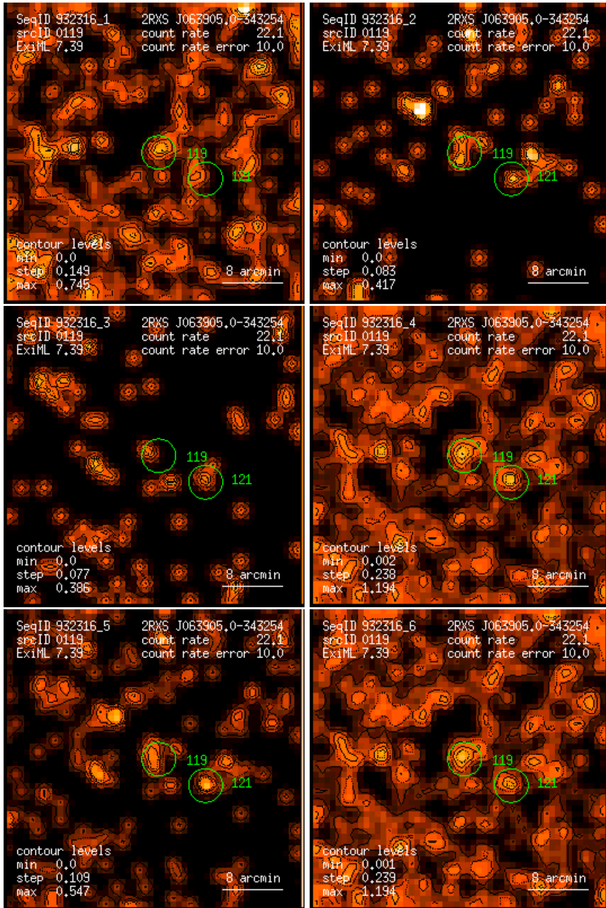
Figure 119: RASS 932316: detection 0119: band rate images, Gaussian filter: (1) PSPC channels 11 – 41, (2) 52 – 90, (3) 91 – 201, (4) 11 – 235, (5) 52 – 201, (6) 11 – 201. Broad band rates in counts/ks. Band rate contour levels in counts/ks/arcmin 2 .
