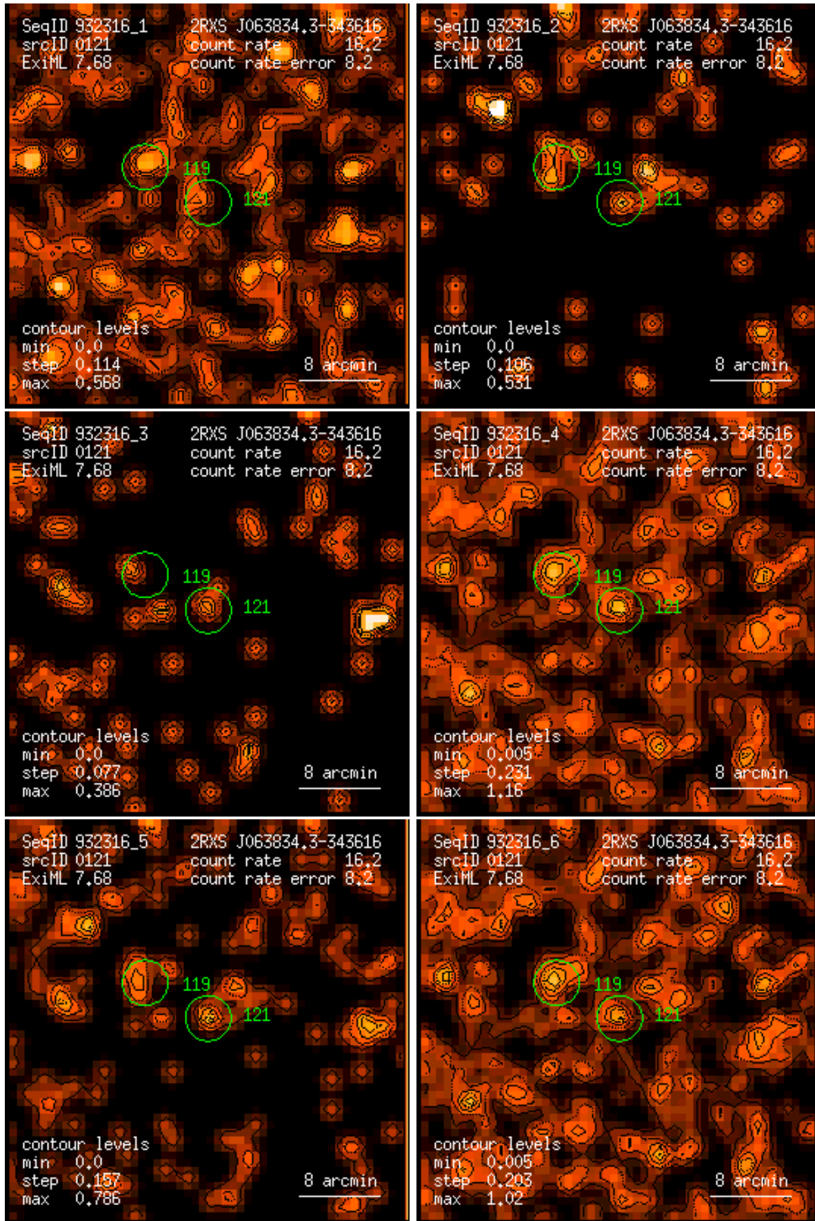
Figure 121: RASS 932316: detection 0121: band rate images, Gaussian filter: (1) PSPC channels 11 – 41, (2) 52 – 90, (3) 91 – 201, (4) 11 – 235, (5) 52 – 201, (6) 11 – 201. Broad band rates in counts/ks. Band rate contour levels in counts/ks/arcmin 2 .
