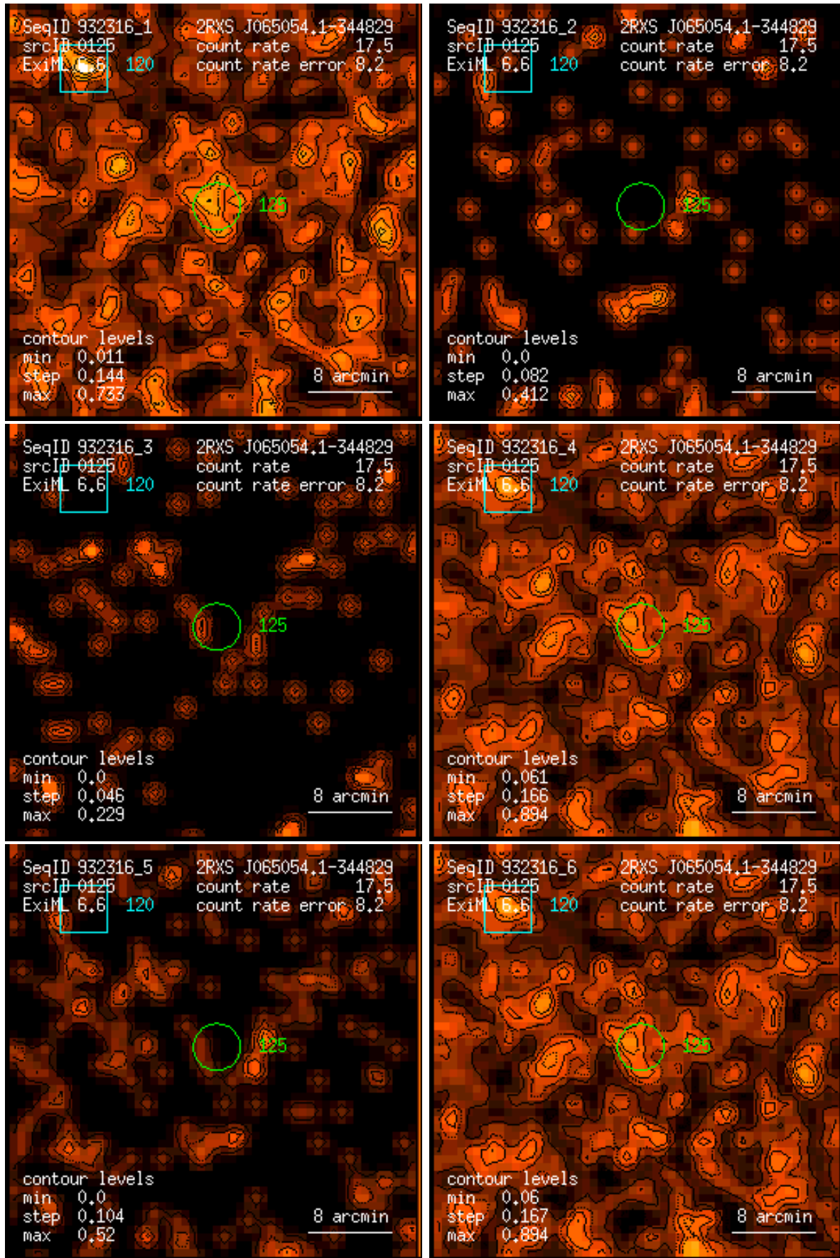
Figure 125: RASS 932316: detection 0125: band rate images, Gaussian filter: (1) PSPC channels 11 – 41, (2) 52 – 90, (3) 91 – 201, (4) 11 – 235, (5) 52 – 201, (6) 11 – 201. Broad band rates in counts/ks. Band rate contour levels in counts/ks/arcmin 2 .
