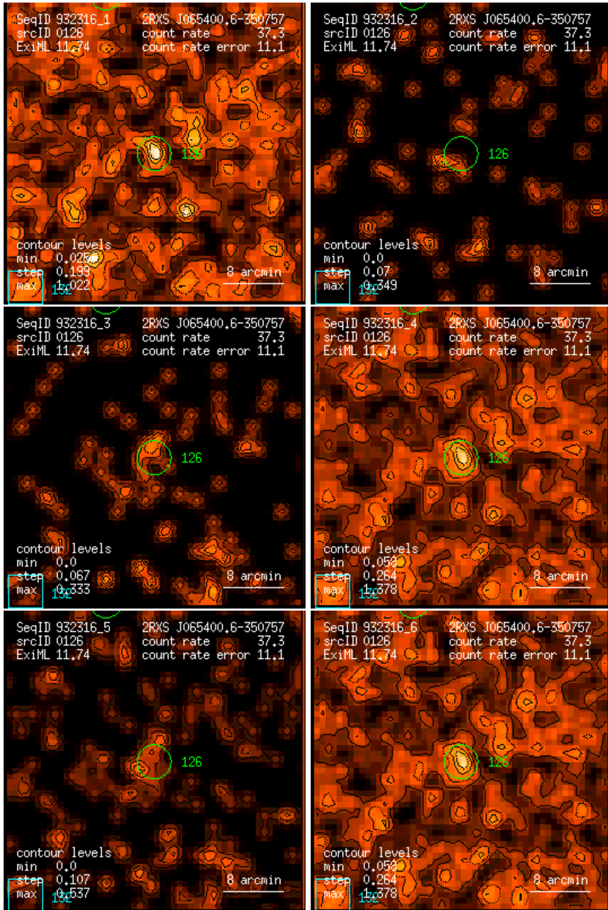
Figure 126: RASS 932316: detection 0126: band rate images, Gaussian filter: (1) PSPC channels 11 – 41, (2) 52 – 90, (3) 91 – 201, (4) 11 – 235, (5) 52 – 201, (6) 11 – 201. Broad band rates in counts/ks. Band rate contour levels in counts/ks/arcmin 2 .
