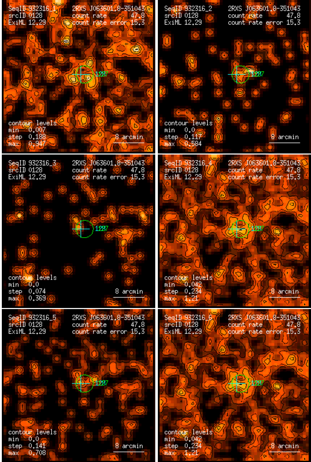
Figure 128: RASS 932316: detection 0128: band rate images, Gaussian filter: (1) PSPC channels 11 – 41, (2) 52 – 90, (3) 91 – 201, (4) 11 – 235, (5) 52 – 201, (6) 11 – 201. Broad band rates in counts/ks. Band rate contour levels in counts/ks/arcmin 2 .
