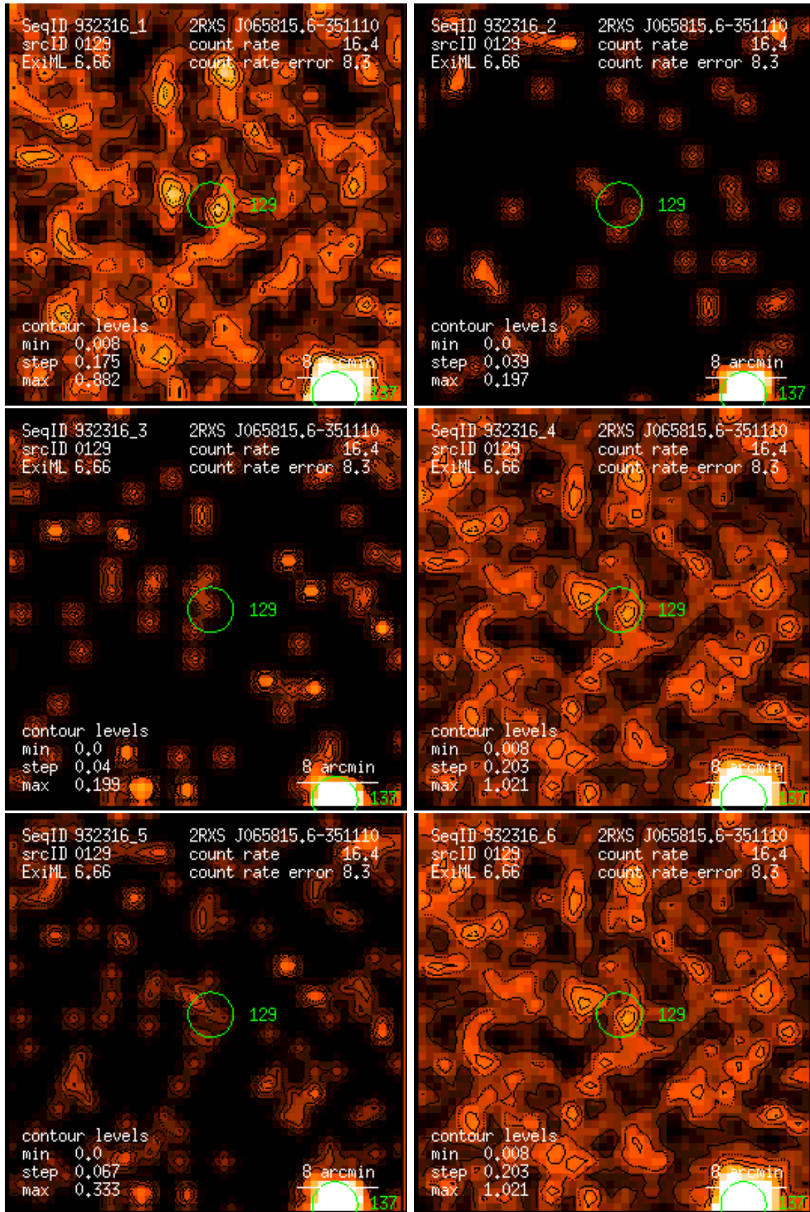
Figure 129: RASS 932316: detection 0129: band rate images, Gaussian filter: (1) PSPC channels 11 – 41, (2) 52 – 90, (3) 91 – 201, (4) 11 – 235, (5) 52 – 201, (6) 11 – 201. Broad band rates in counts/ks. Band rate contour levels in counts/ks/arcmin 2 .
