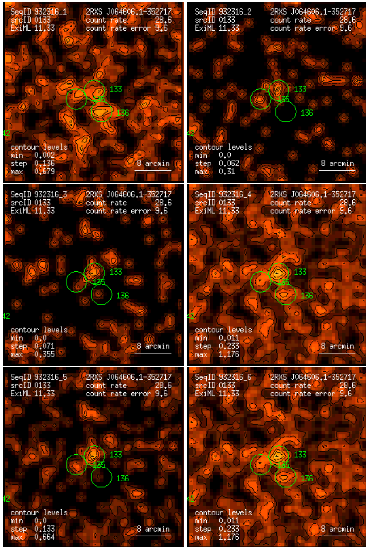
Figure 133: RASS 932316: detection 0133: band rate images, Gaussian filter: (1) PSPC channels 11 – 41, (2) 52 – 90, (3) 91 – 201, (4) 11 – 235, (5) 52 – 201, (6) 11 – 201. Broad band rates in counts/ks. Band rate contour levels in counts/ks/arcmin 2 .
