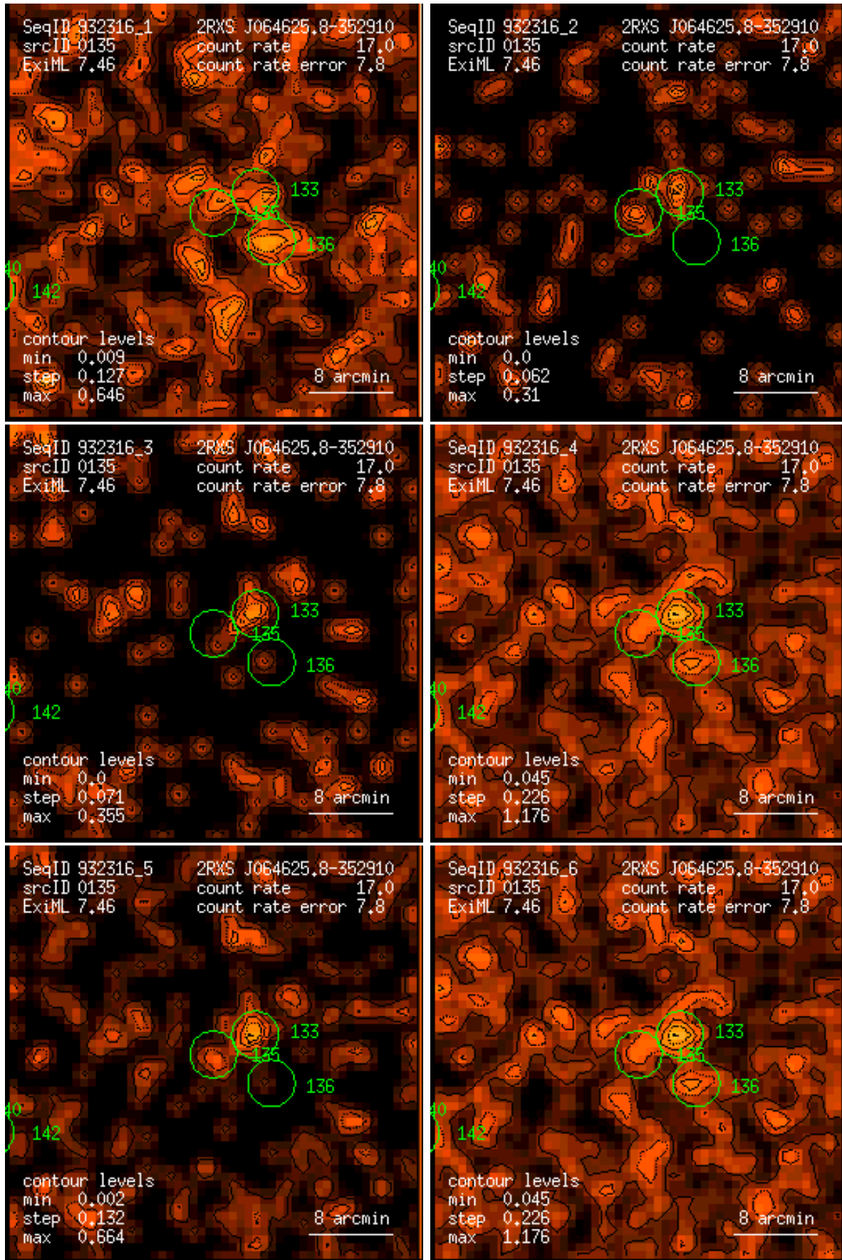
Figure 135: RASS 932316: detection 0135: band rate images, Gaussian filter: (1) PSPC channels 11 – 41, (2) 52 – 90, (3) 91 – 201, (4) 11 – 235, (5) 52 – 201, (6) 11 – 201. Broad band rates in counts/ks. Band rate contour levels in counts/ks/arcmin 2 .
