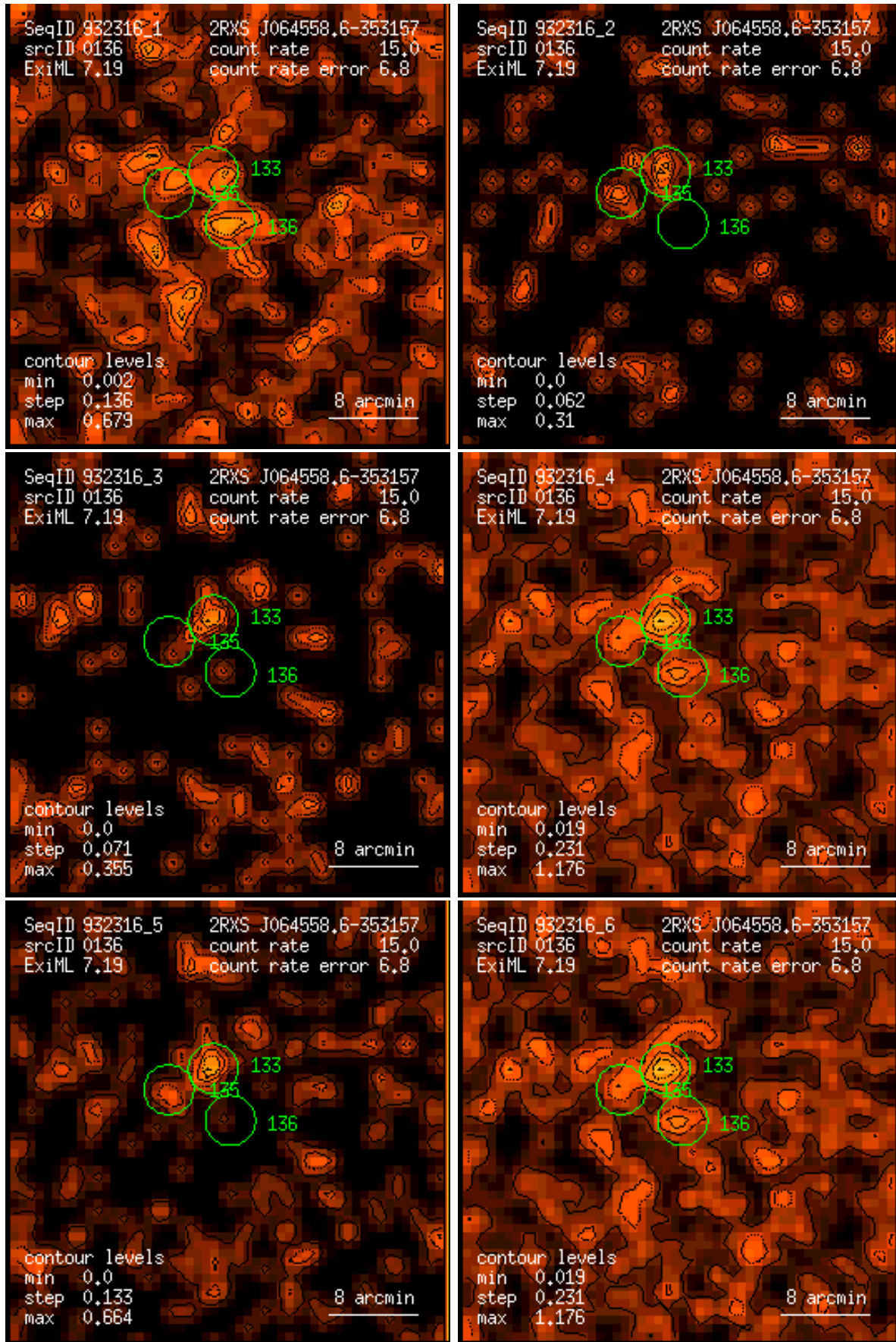
Figure 136: RASS 932316: detection 0136: band rate images, Gaussian filter: (1) PSPC channels 11 – 41, (2) 52 – 90, (3) 91 – 201, (4) 11 – 235, (5) 52 – 201, (6) 11 – 201. Broad band rates in counts/ks. Band rate contour levels in counts/ks/arcmin 2 .
