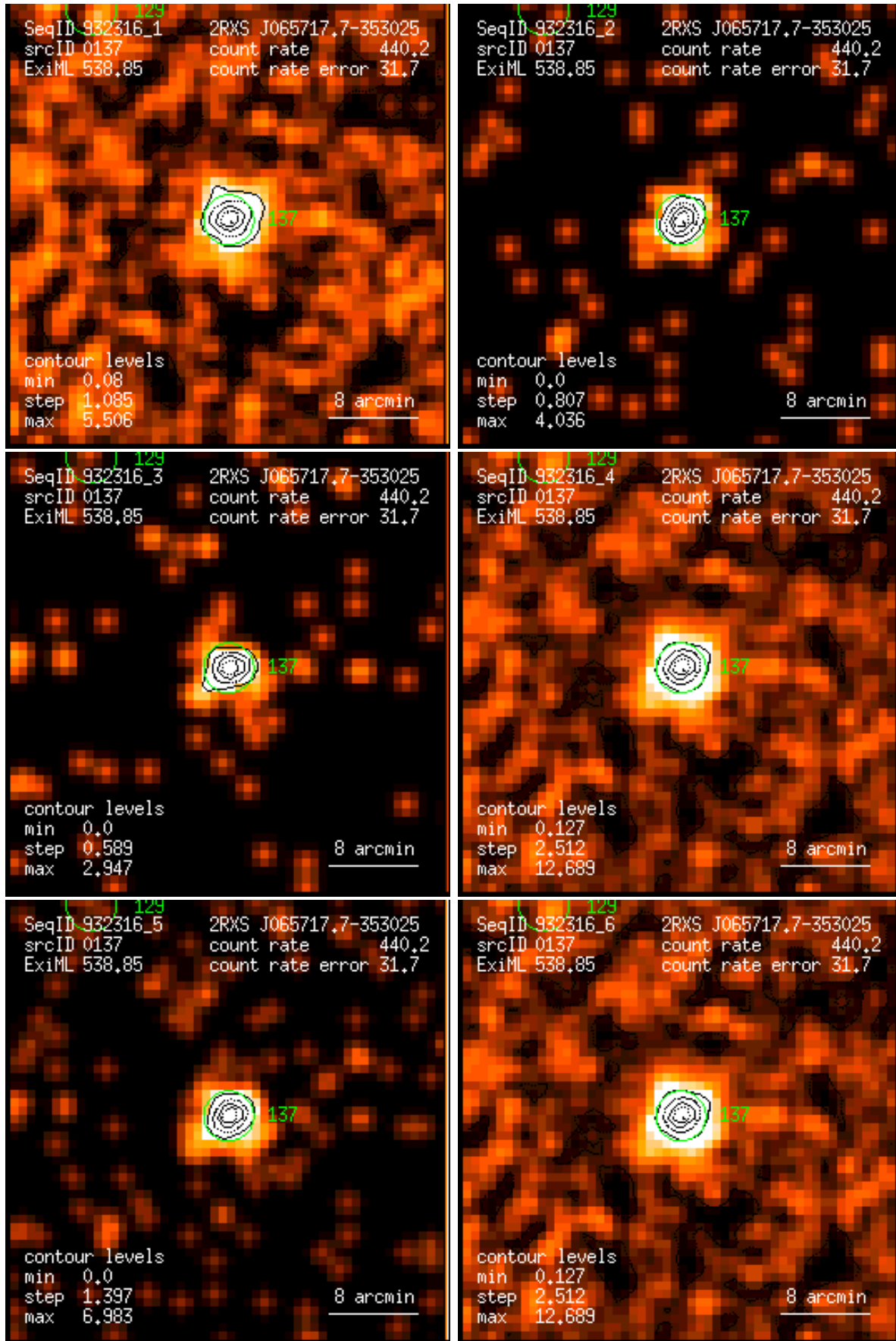
Figure 137: RASS 932316: detection 0137: band rate images, Gaussian filter: (1) PSPC channels 11 – 41, (2) 52 – 90, (3) 91 – 201, (4) 11 – 235, (5) 52 – 201, (6) 11 – 201. Broad band rates in counts/ks. Band rate contour levels in counts/ks/arcmin 2 .
