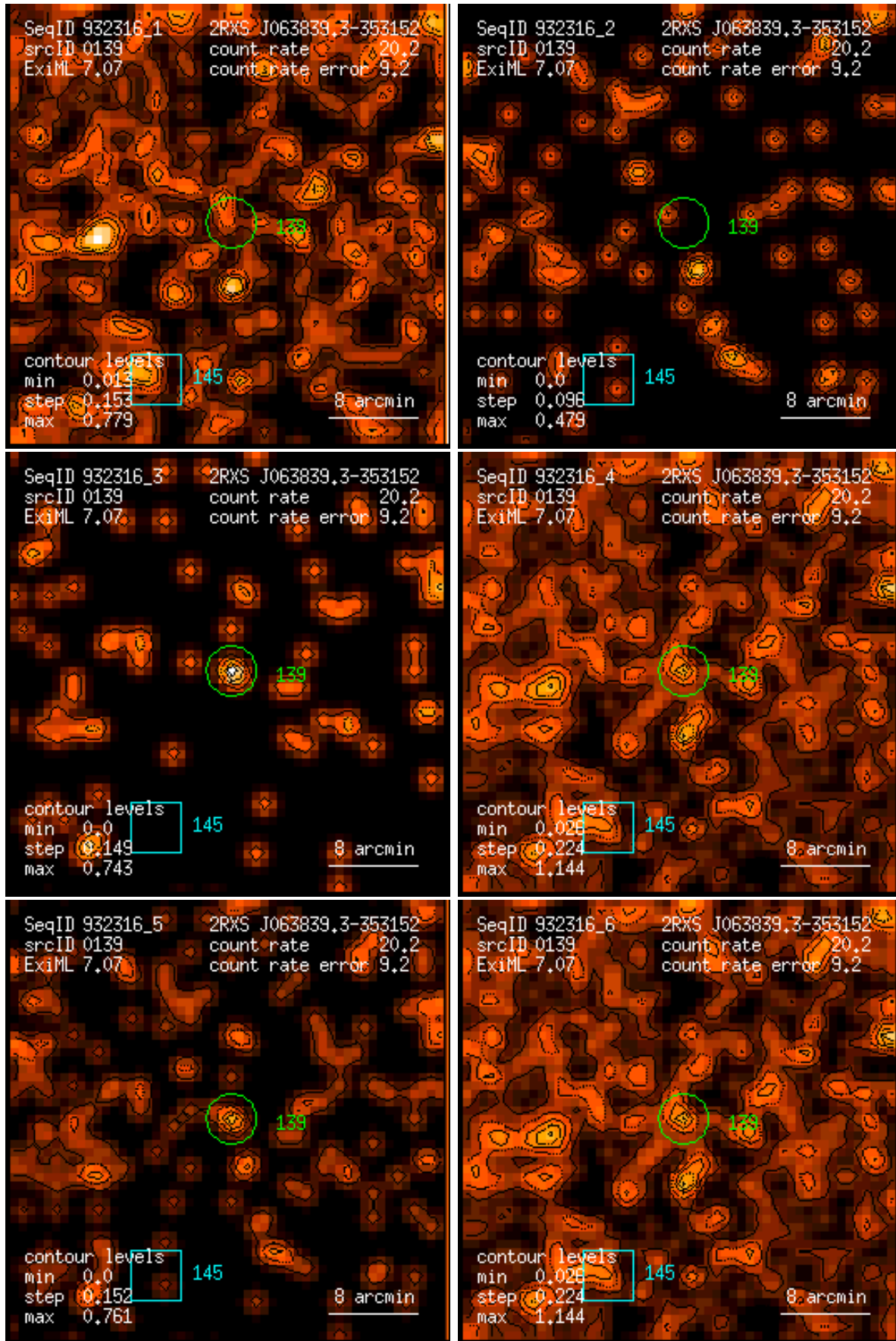
Figure 139: RASS 932316: detection 0139: band rate images, Gaussian filter: (1) PSPC channels 11 – 41, (2) 52 – 90, (3) 91 – 201, (4) 11 – 235, (5) 52 – 201, (6) 11 – 201. Broad band rates in counts/ks. Band rate contour levels in counts/ks/arcmin 2 .
