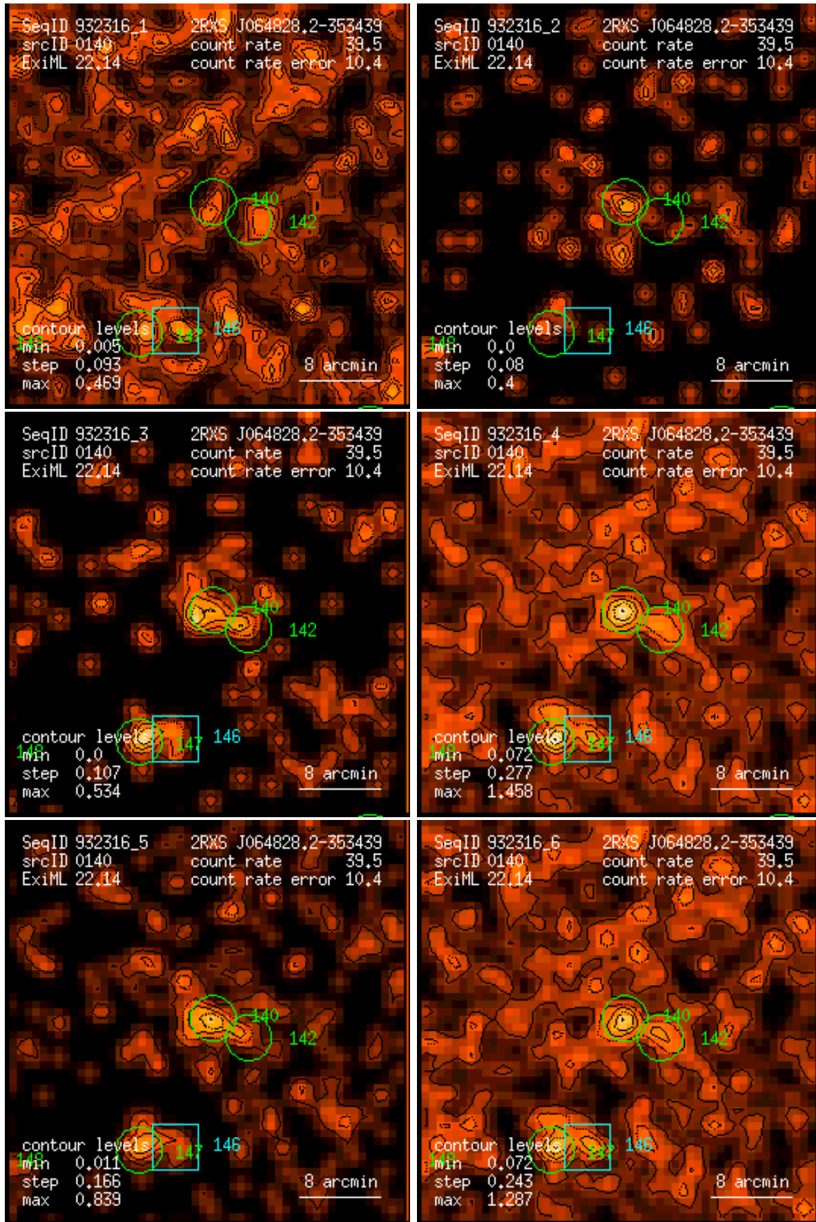
Figure 140: RASS 932316: detection 0140: band rate images, Gaussian filter: (1) PSPC channels 11 – 41, (2) 52 – 90, (3) 91 – 201, (4) 11 – 235, (5) 52 – 201, (6) 11 – 201. Broad band rates in counts/ks. Band rate contour levels in counts/ks/arcmin 2 .
