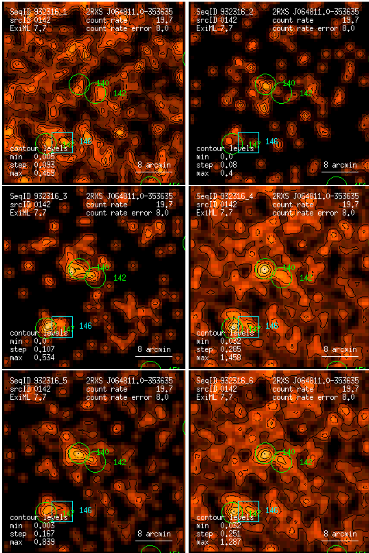
Figure 142: RASS 932316: detection 0142: band rate images, Gaussian filter: (1) PSPC channels 11 – 41, (2) 52 – 90, (3) 91 – 201, (4) 11 – 235, (5) 52 – 201, (6) 11 – 201. Broad band rates in counts/ks. Band rate contour levels in counts/ks/arcmin 2 .
