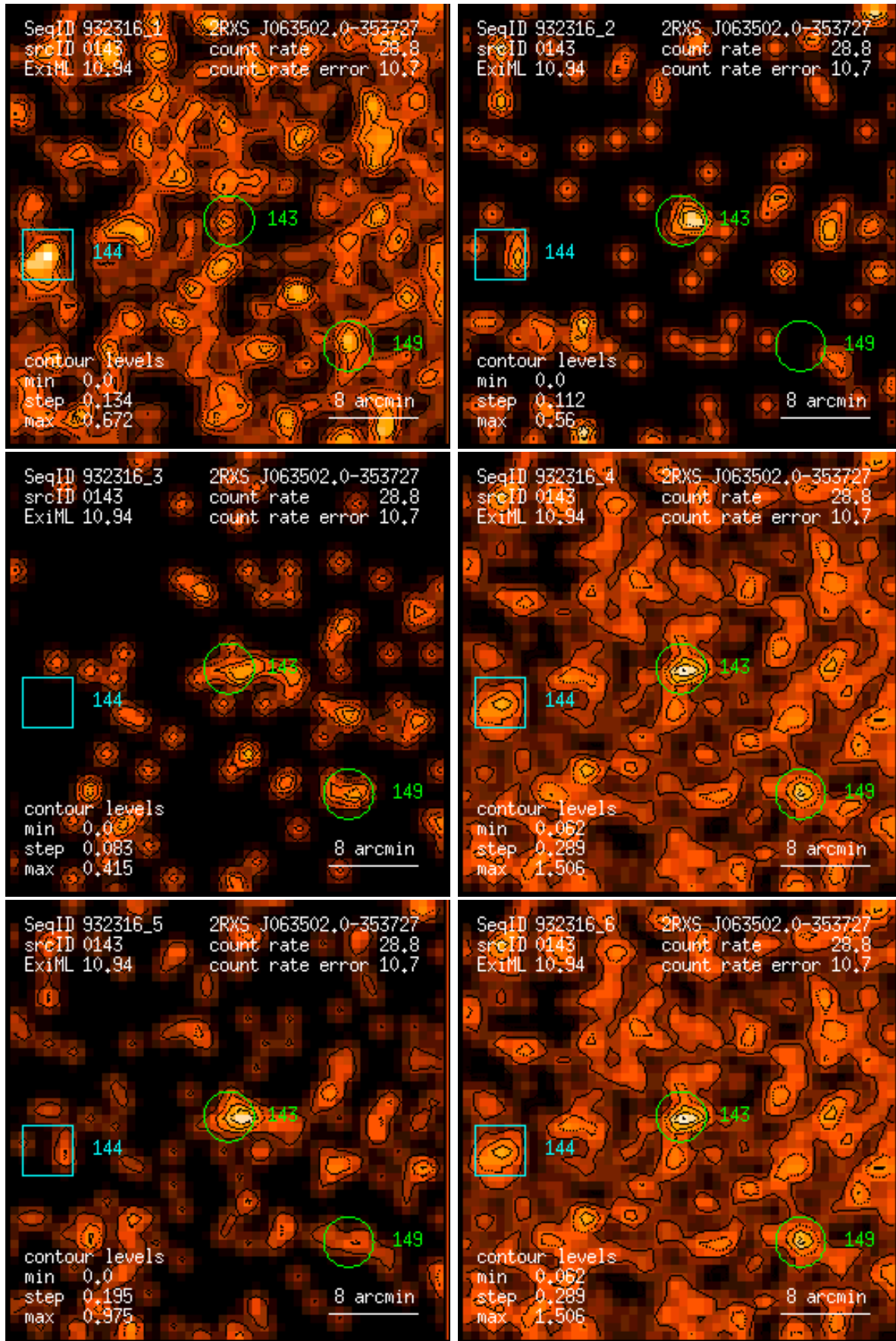
Figure 143: RASS 932316: detection 0143: band rate images, Gaussian filter: (1) PSPC channels 11 – 41, (2) 52 – 90, (3) 91 – 201, (4) 11 – 235, (5) 52 – 201, (6) 11 – 201. Broad band rates in counts/ks. Band rate contour levels in counts/ks/arcmin 2 .
