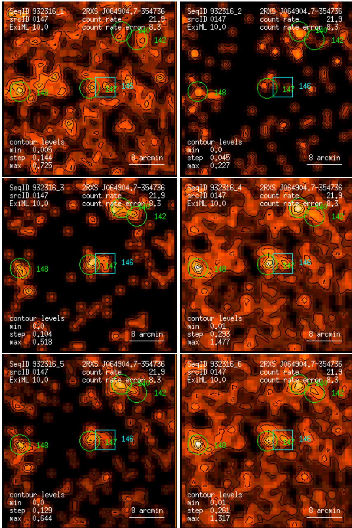
Figure 147: RASS 932316: detection 0147: band rate images, Gaussian filter: (1) PSPC channels 11 – 41, (2) 52 – 90, (3) 91 – 201, (4) 11 – 235, (5) 52 – 201, (6) 11 – 201. Broad band rates in counts/ks. Band rate contour levels in counts/ks/arcmin 2 .
