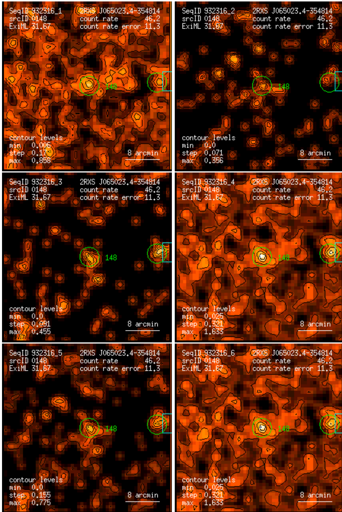
Figure 148: RASS 932316: detection 0148: band rate images, Gaussian filter: (1) PSPC channels 11 – 41, (2) 52 – 90, (3) 91 – 201, (4) 11 – 235, (5) 52 – 201, (6) 11 – 201. Broad band rates in counts/ks. Band rate contour levels in counts/ks/arcmin 2 .
