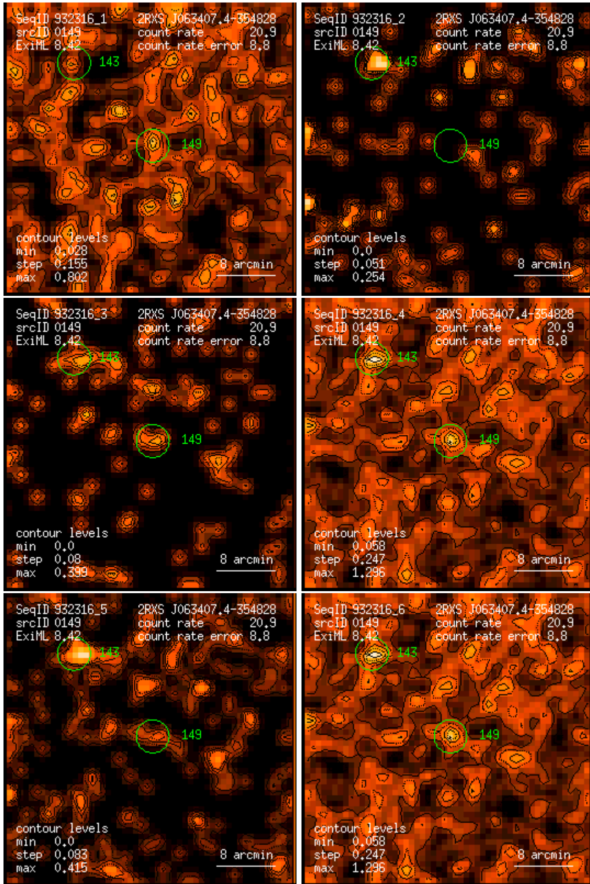
Figure 149: RASS 932316: detection 0149: band rate images, Gaussian filter: (1) PSPC channels 11 – 41, (2) 52 – 90, (3) 91 – 201, (4) 11 – 235, (5) 52 – 201, (6) 11 – 201. Broad band rates in counts/ks. Band rate contour levels in counts/ks/arcmin 2 .
