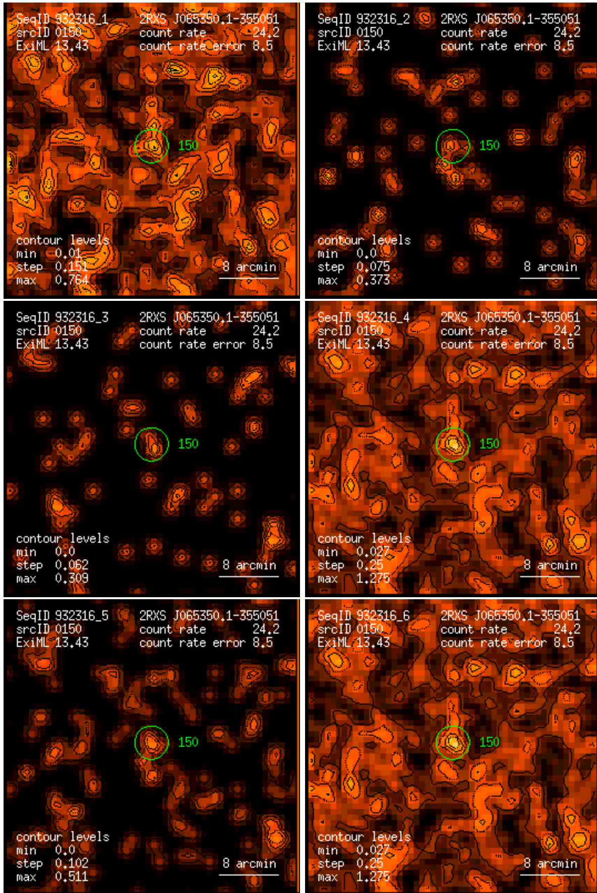
Figure 150: RASS 932316: detection 0150: band rate images, Gaussian filter: (1) PSPC channels 11 – 41, (2) 52 – 90, (3) 91 – 201, (4) 11 – 235, (5) 52 – 201, (6) 11 – 201. Broad band rates in counts/ks. Band rate contour levels in counts/ks/arcmin 2 .
