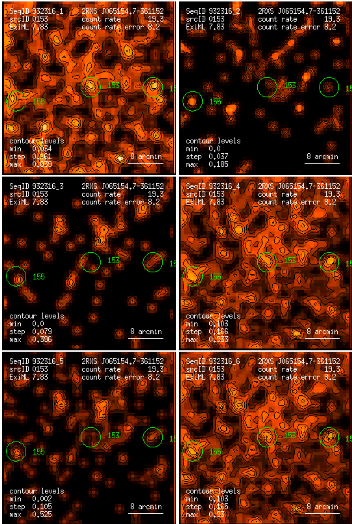
Figure 153: RASS 932316: detection 0153: band rate images, Gaussian filter: (1) PSPC channels 11 – 41, (2) 52 – 90, (3) 91 – 201, (4) 11 – 235, (5) 52 – 201, (6) 11 – 201. Broad band rates in counts/ks. Band rate contour levels in counts/ks/arcmin 2 .
