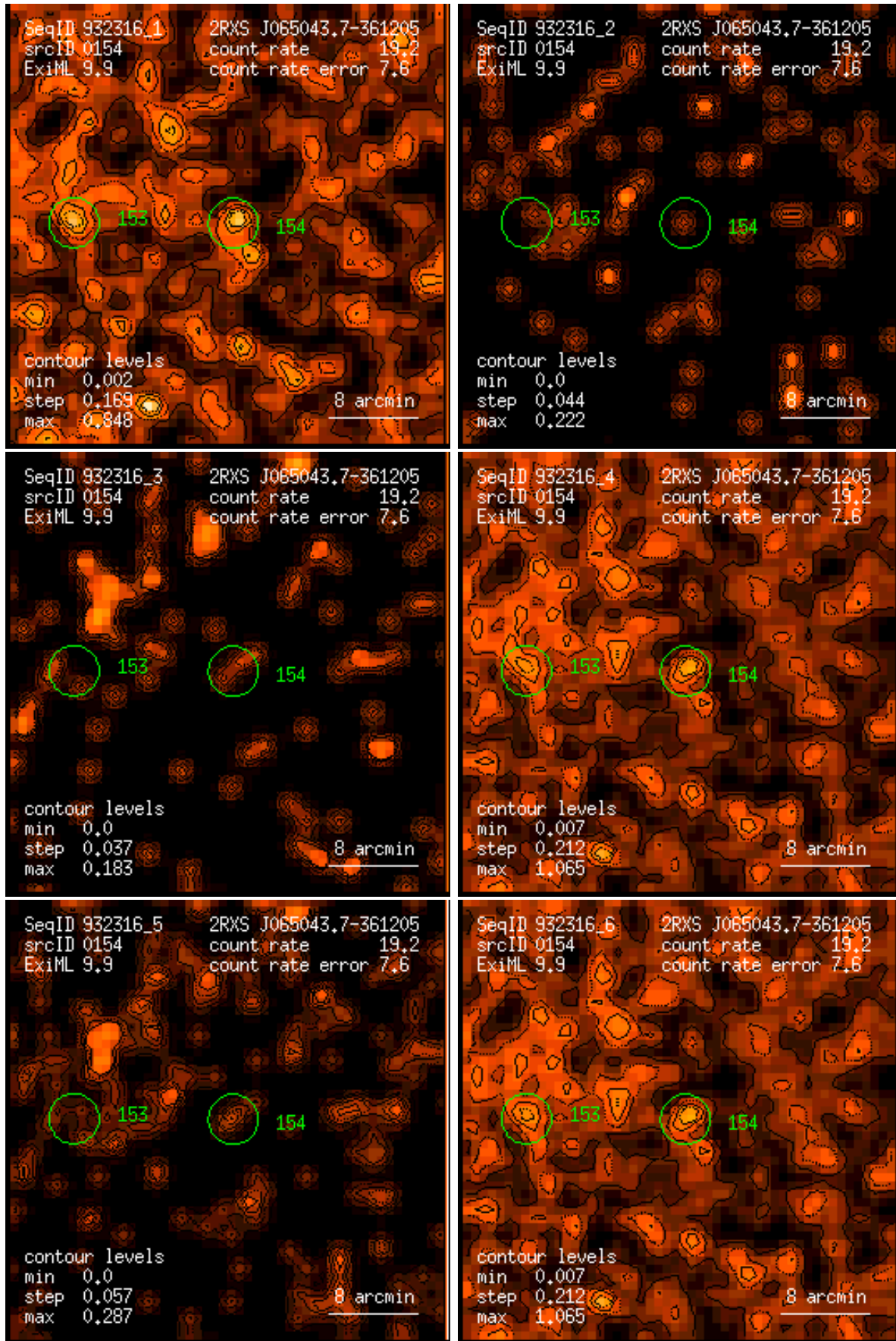
Figure 154: RASS 932316: detection 0154: band rate images, Gaussian filter: (1) PSPC channels 11 – 41, (2) 52 – 90, (3) 91 – 201, (4) 11 – 235, (5) 52 – 201, (6) 11 – 201. Broad band rates in counts/ks. Band rate contour levels in counts/ks/arcmin 2 .
