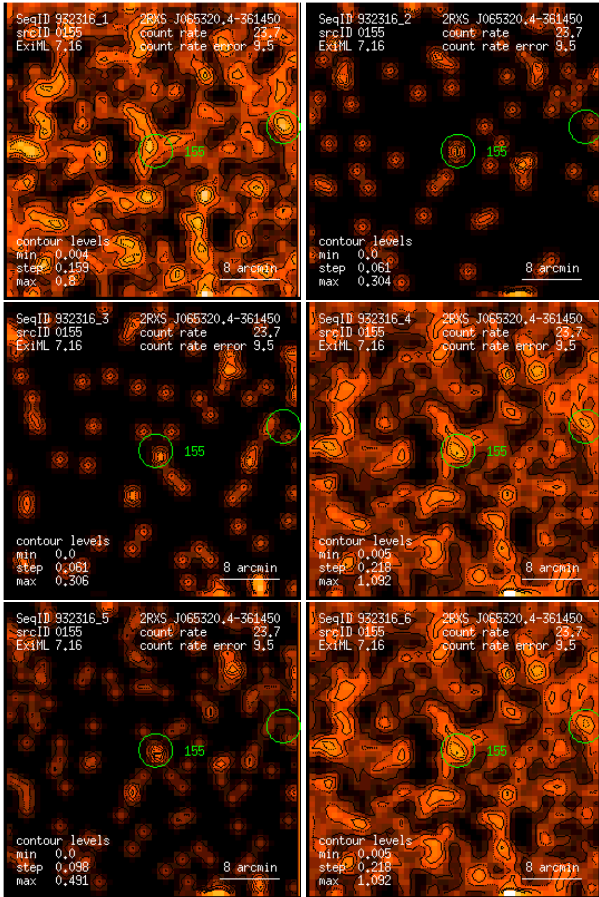
Figure 155: RASS 932316: detection 0155: band rate images, Gaussian filter: (1) PSPC channels 11 – 41, (2) 52 – 90, (3) 91 – 201, (4) 11 – 235, (5) 52 – 201, (6) 11 – 201. Broad band rates in counts/ks. Band rate contour levels in counts/ks/arcmin 2 .
