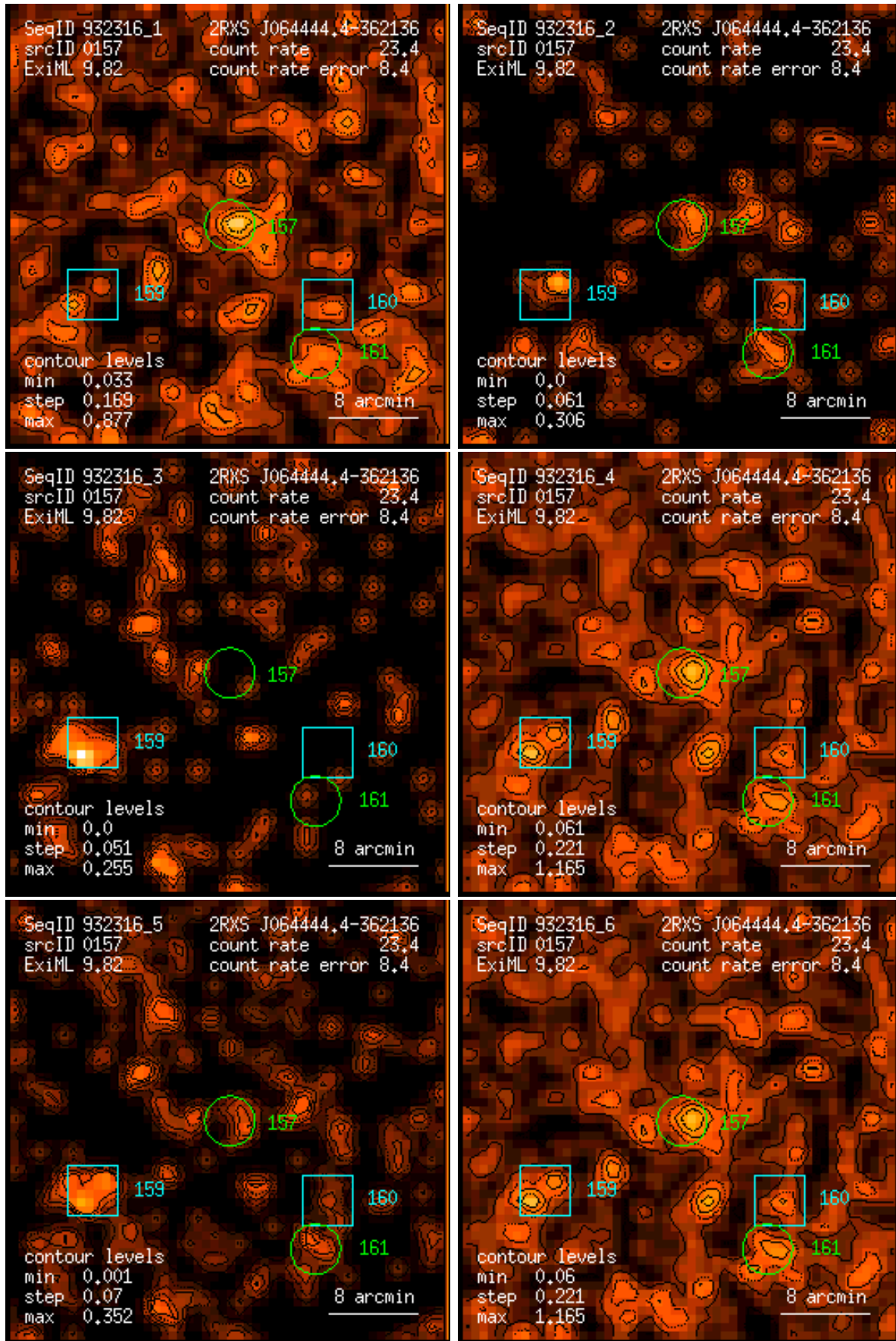
Figure 157: RASS 932316: detection 0157: band rate images, Gaussian filter: (1) PSPC channels 11 – 41, (2) 52 – 90, (3) 91 – 201, (4) 11 – 235, (5) 52 – 201, (6) 11 – 201. Broad band rates in counts/ks. Band rate contour levels in counts/ks/arcmin 2 .
