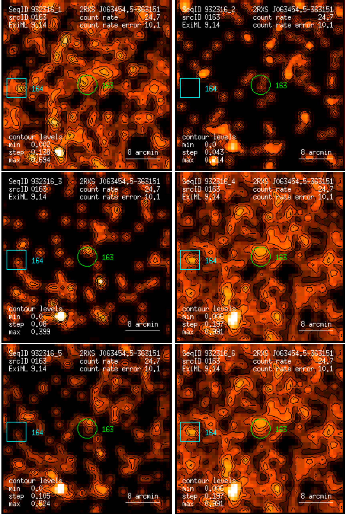
Figure 163: RASS 932316: detection 0163: band rate images, Gaussian filter: (1) PSPC channels 11 – 41, (2) 52 – 90, (3) 91 – 201, (4) 11 – 235, (5) 52 – 201, (6) 11 – 201. Broad band rates in counts/ks. Band rate contour levels in counts/ks/arcmin 2 .
