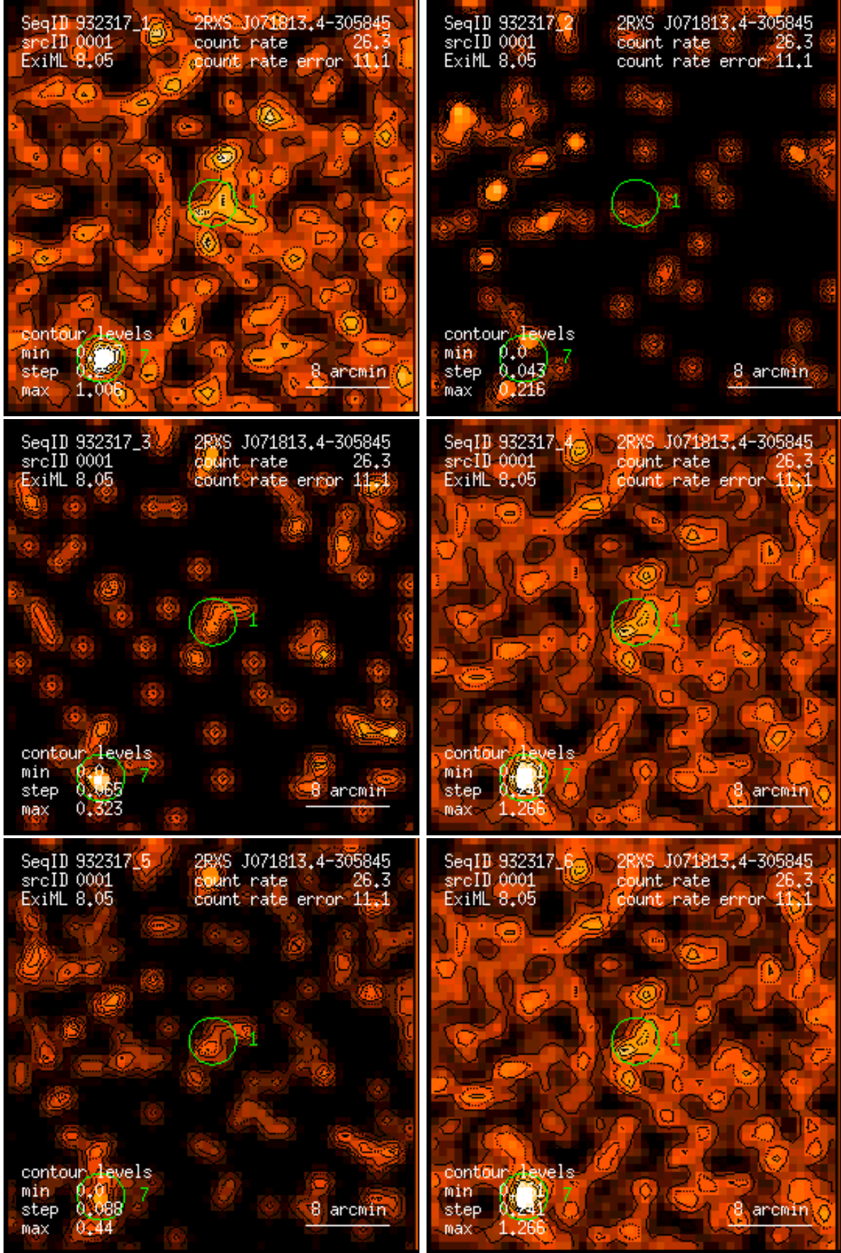
Figure 1: RASS 932317: detection 0001: band rate images, Gaussian filter: (1) PSPC channels 11 – 41, (2) 52 – 90, (3) 91 – 201, (4) 11 – 235, (5) 52 – 201, (6) 11 – 201. Broad band rates in counts/ks. Band rate contour levels in counts/ks/arcmin 2 .
