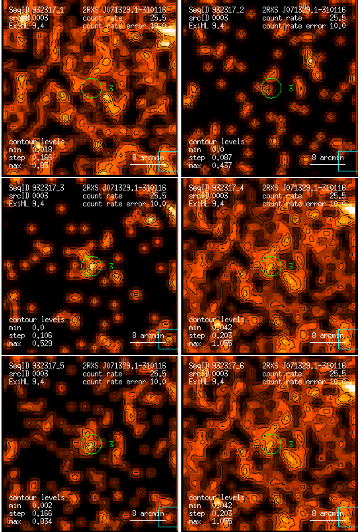
Figure 3: RASS 932317: detection 0003: band rate images, Gaussian filter: (1) PSPC channels 11 – 41, (2) 52 – 90, (3) 91 – 201, (4) 11 – 235, (5) 52 – 201, (6) 11 – 201. Broad band rates in counts/ks. Band rate contour levels in counts/ks/arcmin 2 .
