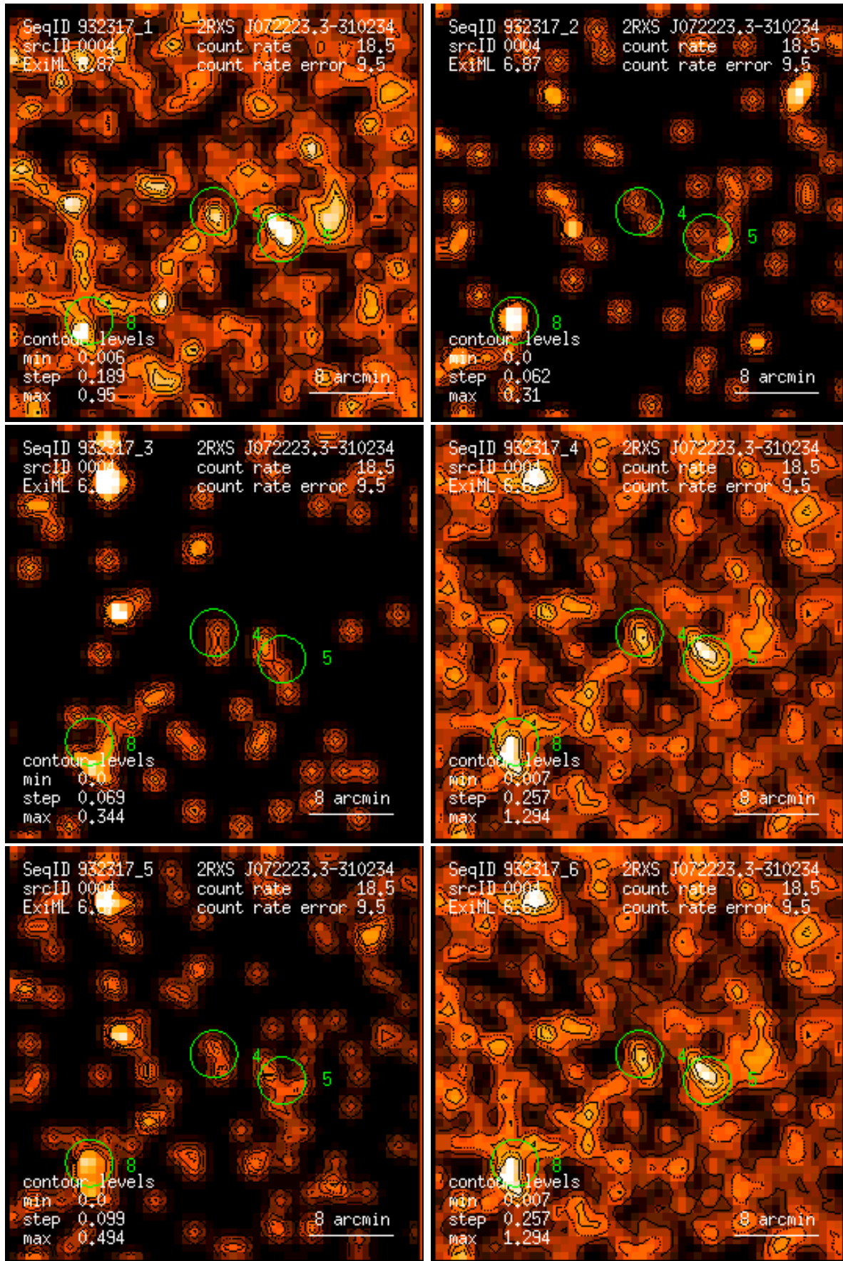
Figure 4: RASS 932317: detection 0004: band rate images, Gaussian filter: (1) PSPC channels 11 – 41, (2) 52 – 90, (3) 91 – 201, (4) 11 – 235, (5) 52 – 201, (6) 11 – 201. Broad band rates in counts/ks. Band rate contour levels in counts/ks/arcmin 2 .
